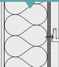
Horizontal Joint
