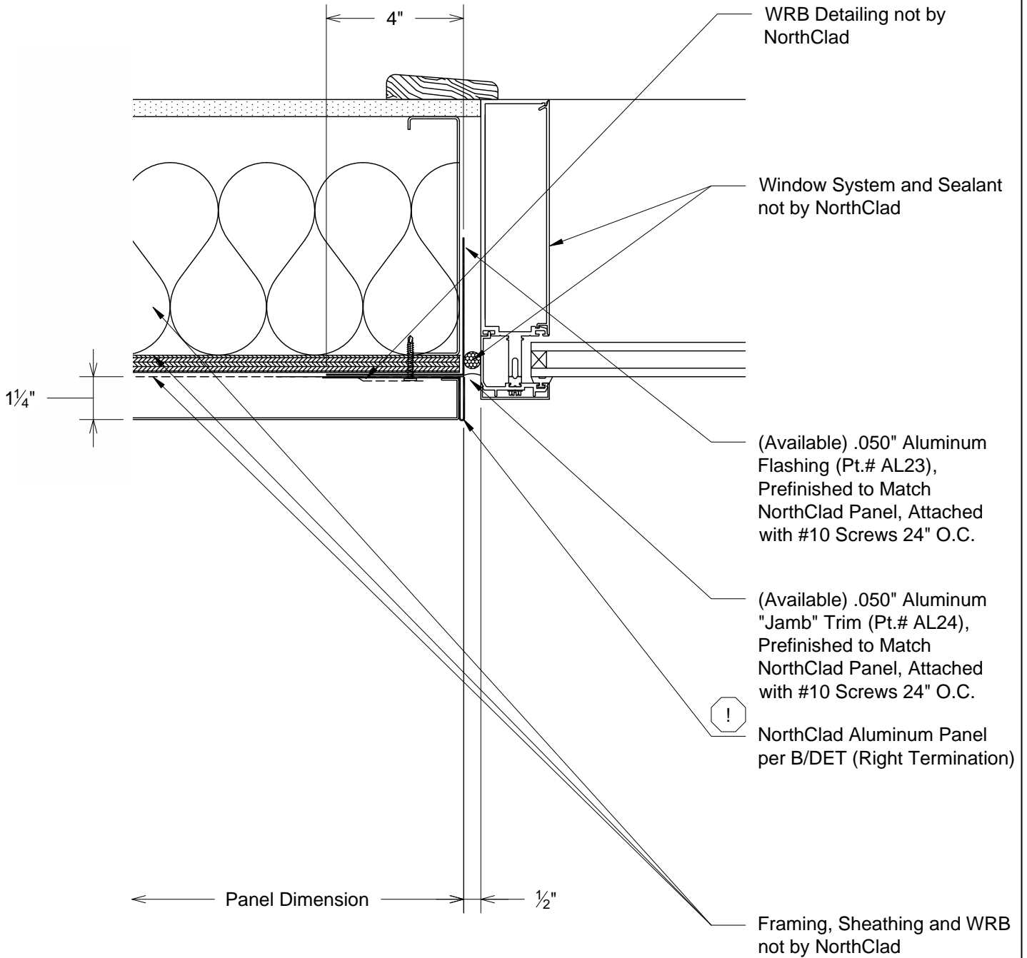
K1 DET Plan - Window at Left Jamb
