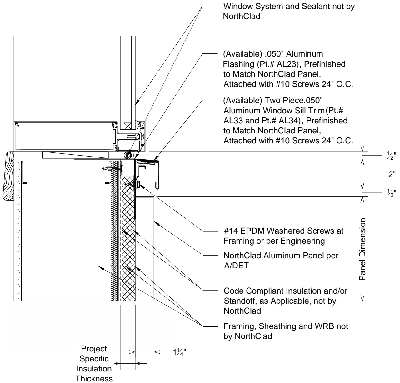
N1 Section - Window Sill DET
