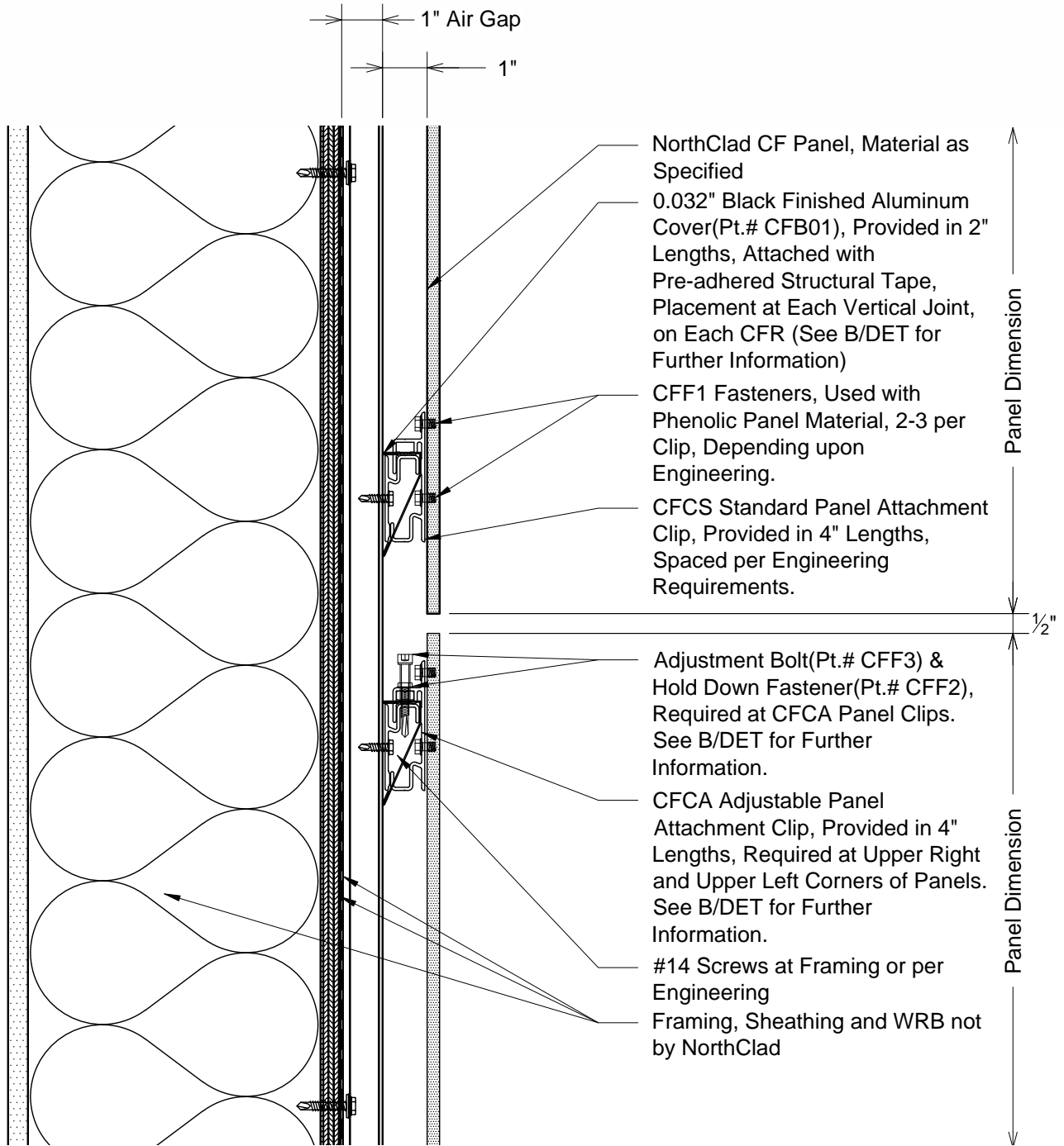
A Section - Horizontal Joint DET With Insulation Inboard of the Stud Cavity
