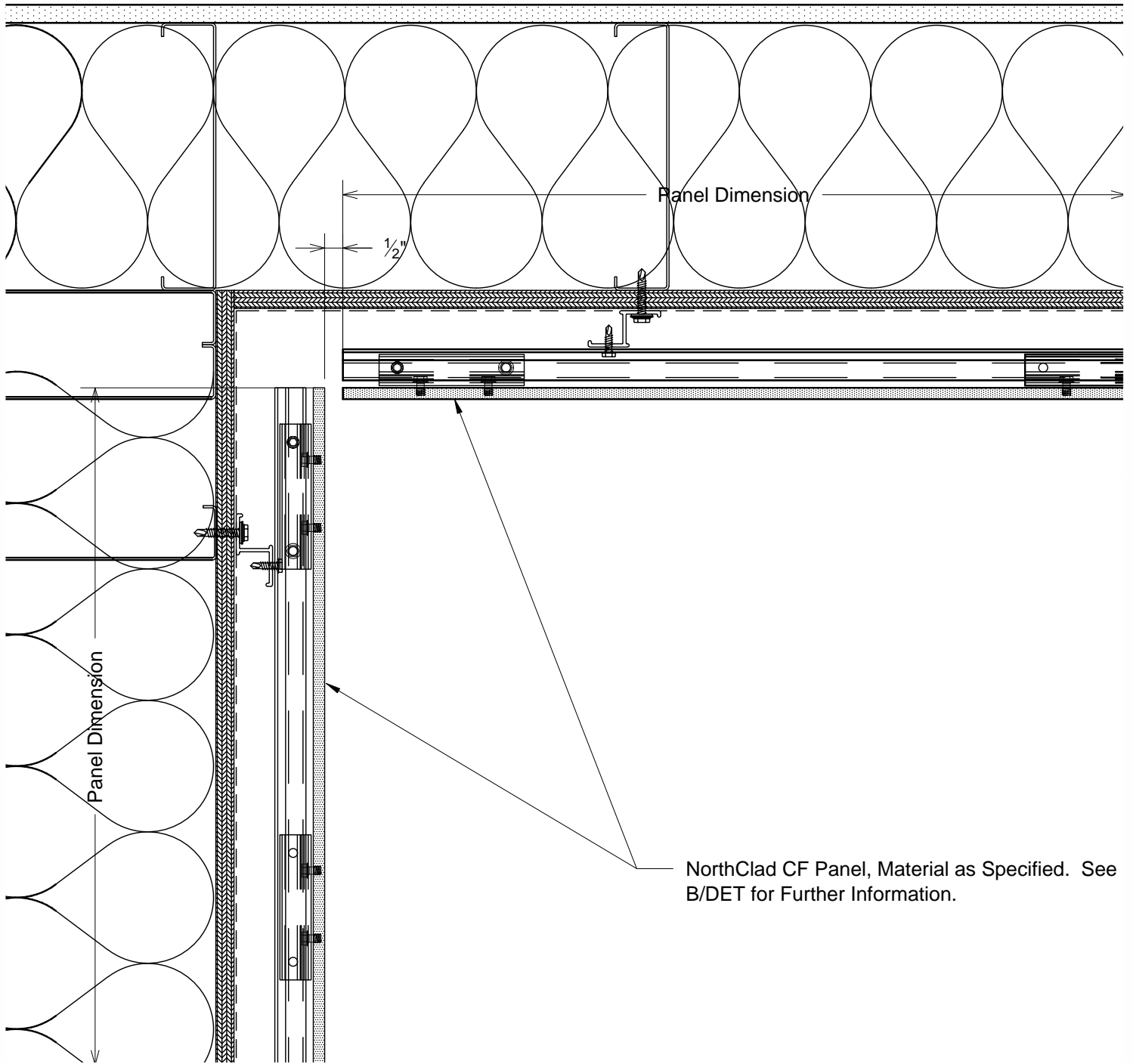
H1 Plan - Inside Corner DET With Insulation Inboard of the Stud Cavity
