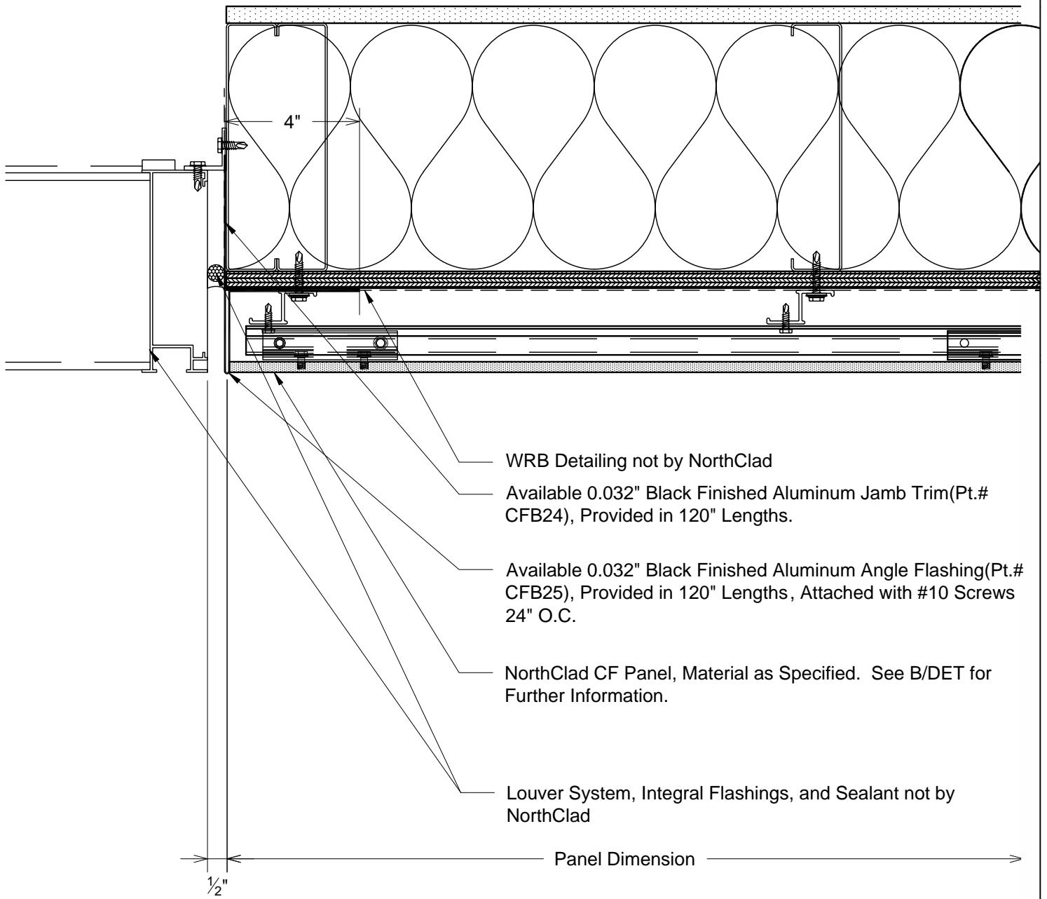
M2 Plan - Louver at Right Jamb DET With Insulation Inboard of the Stud Cavity
