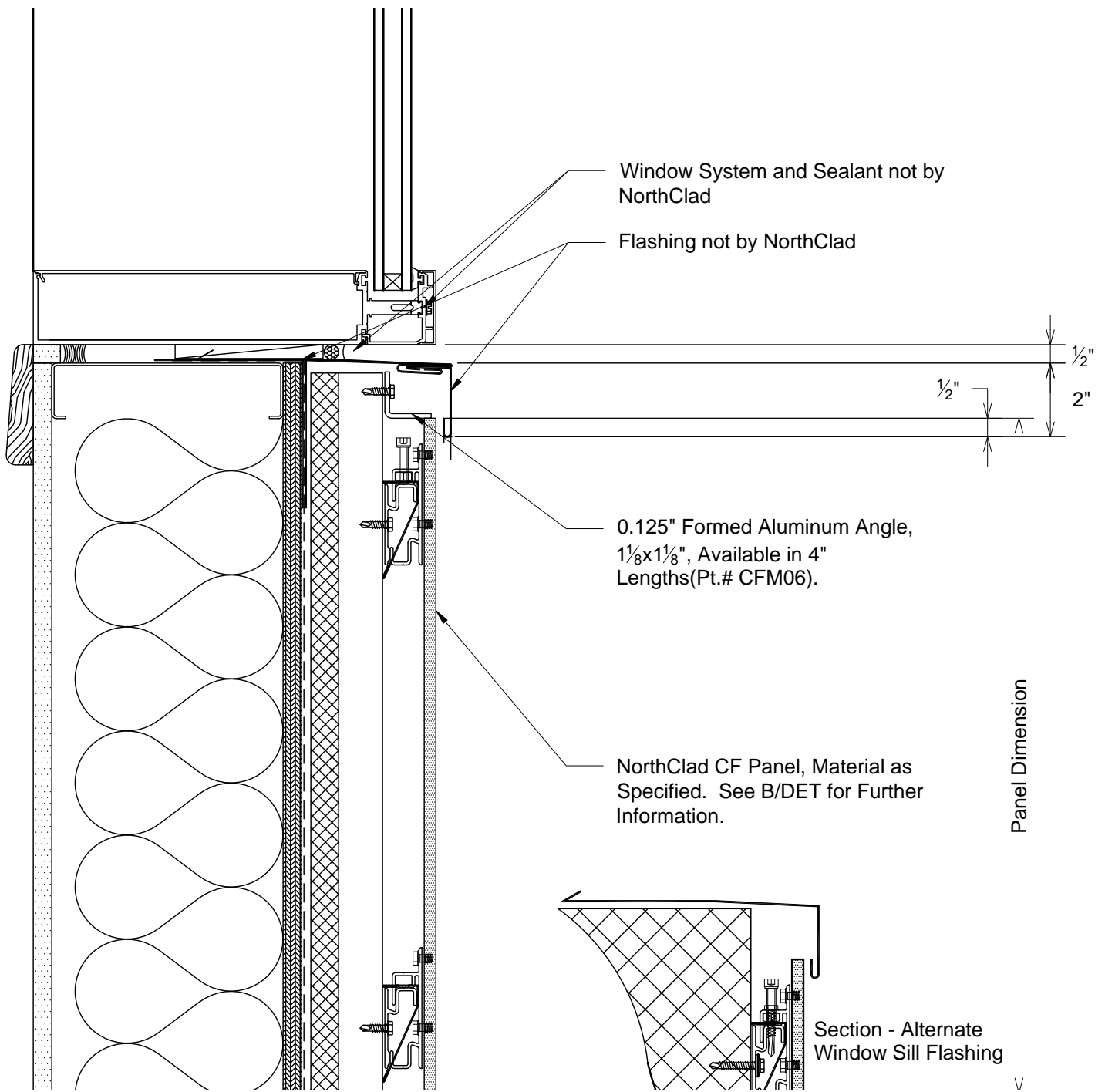
J1 Section - Window Sill DET With Insulation Outboard of Stud Cavity
