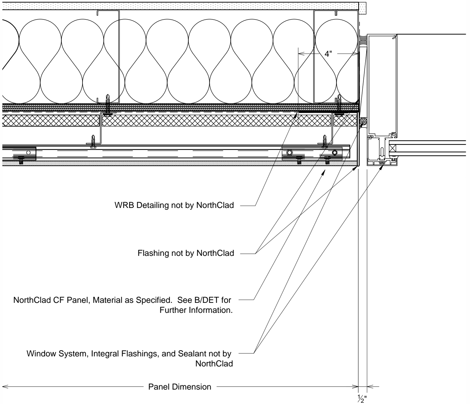
N1 Plan - Window at Left Jamb DET With Insulation Outboard of Stud Cavity
