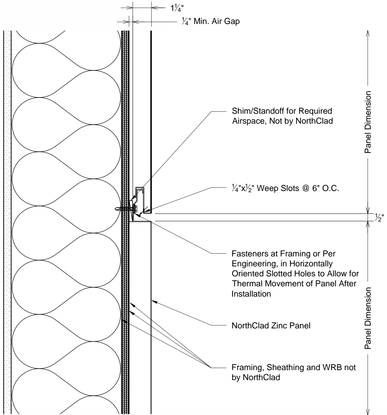
A Section - Horizontal Joint DET
