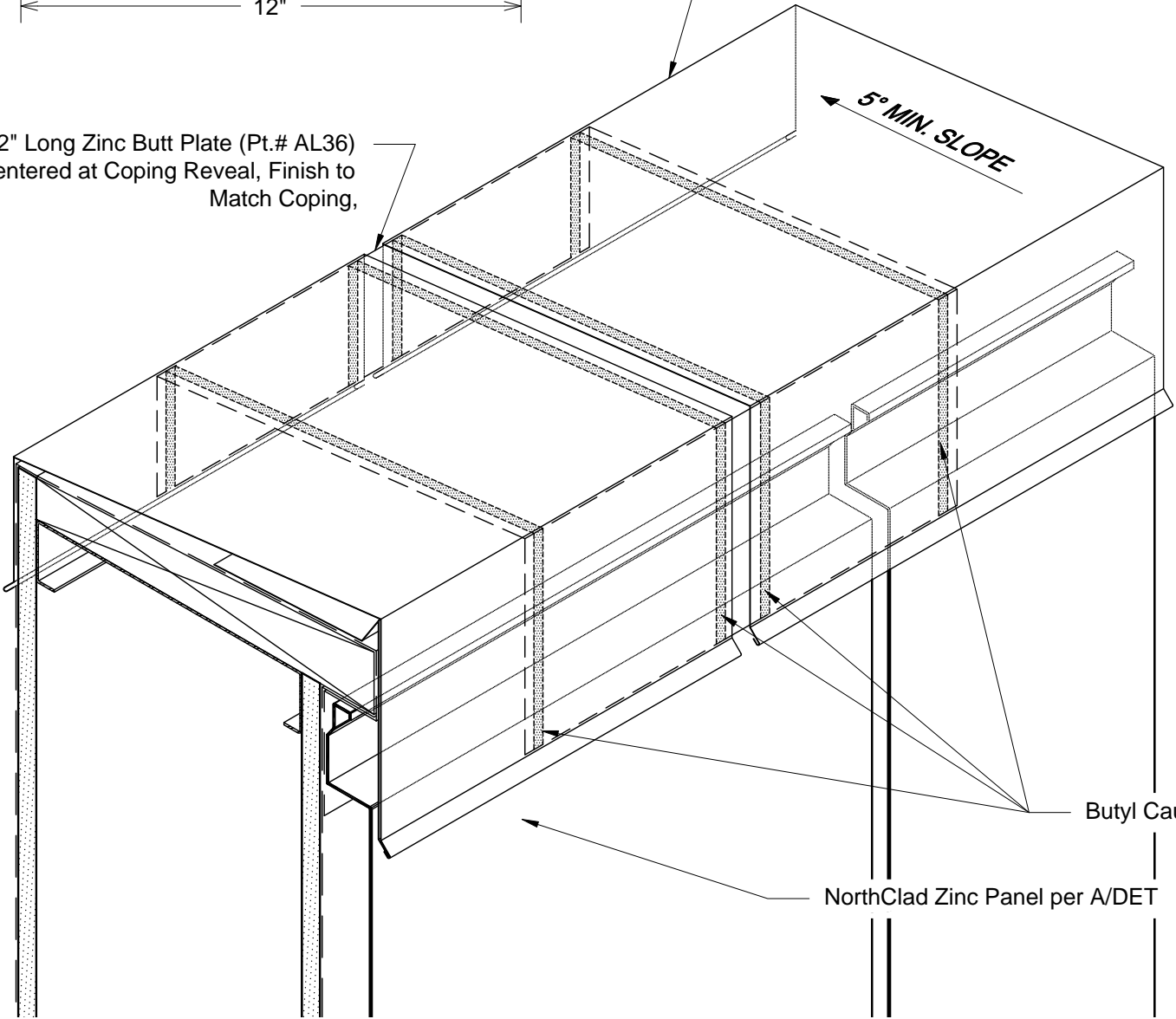
E Isometric - Parapet Coping Splice DET
