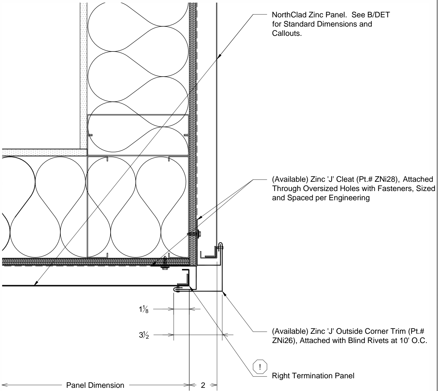
G2 Plan - Outside Corner with Trim DET
