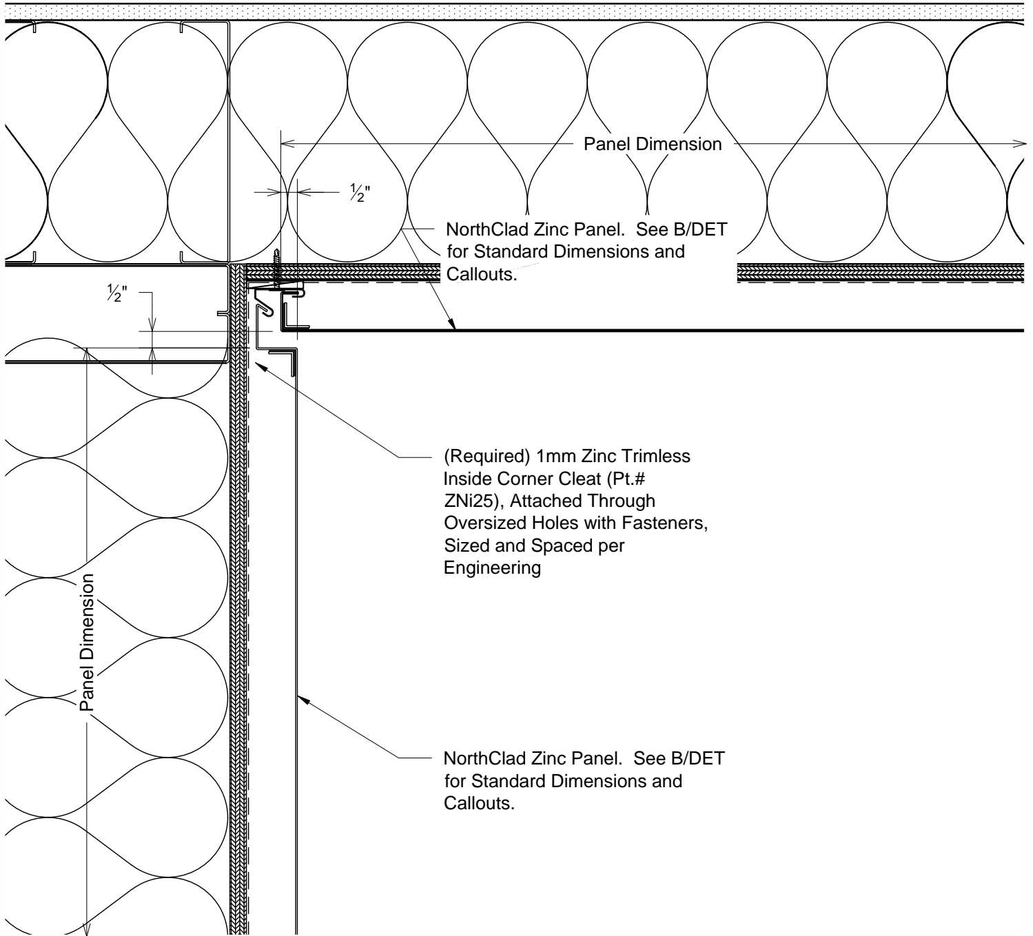
H1 DET Plan - Inside Corner
