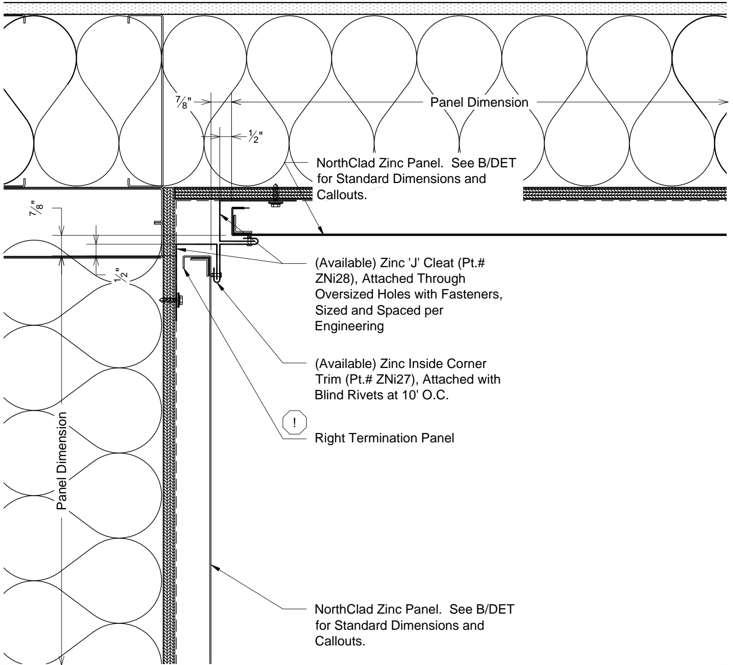
H2 DET Plan - Inside Corner with Trim
