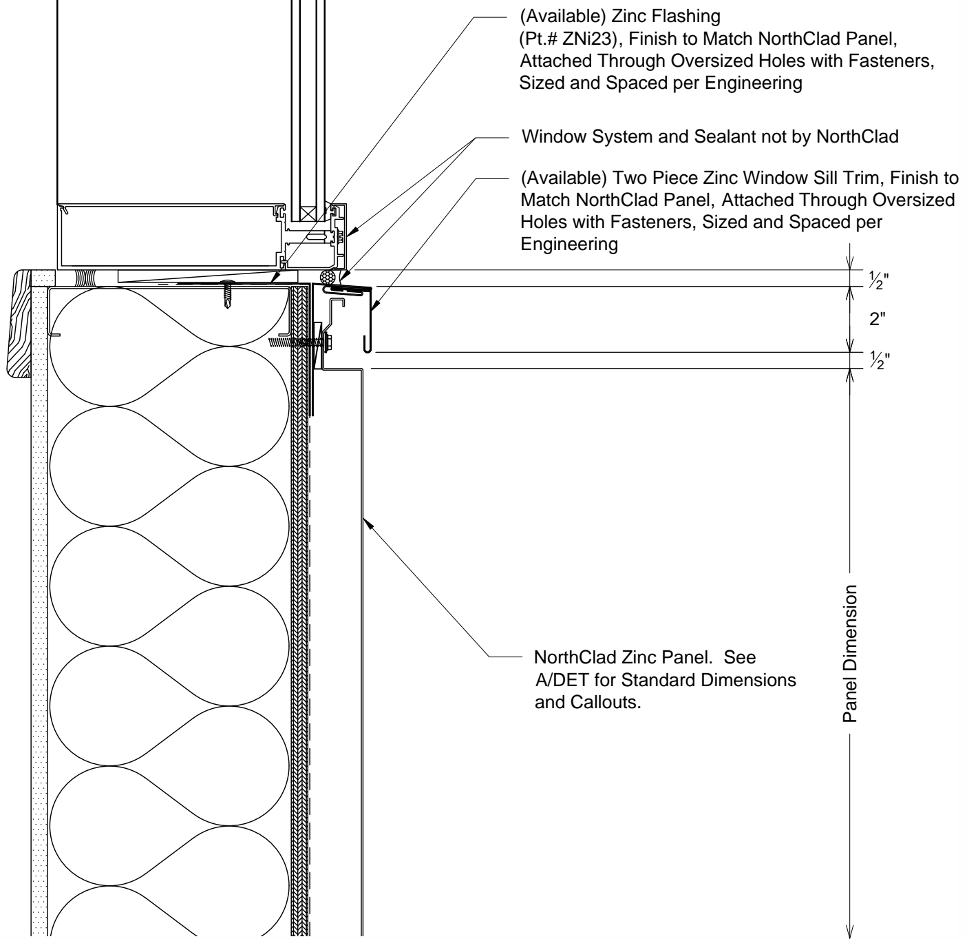
J1 Section - Window Sill DET
