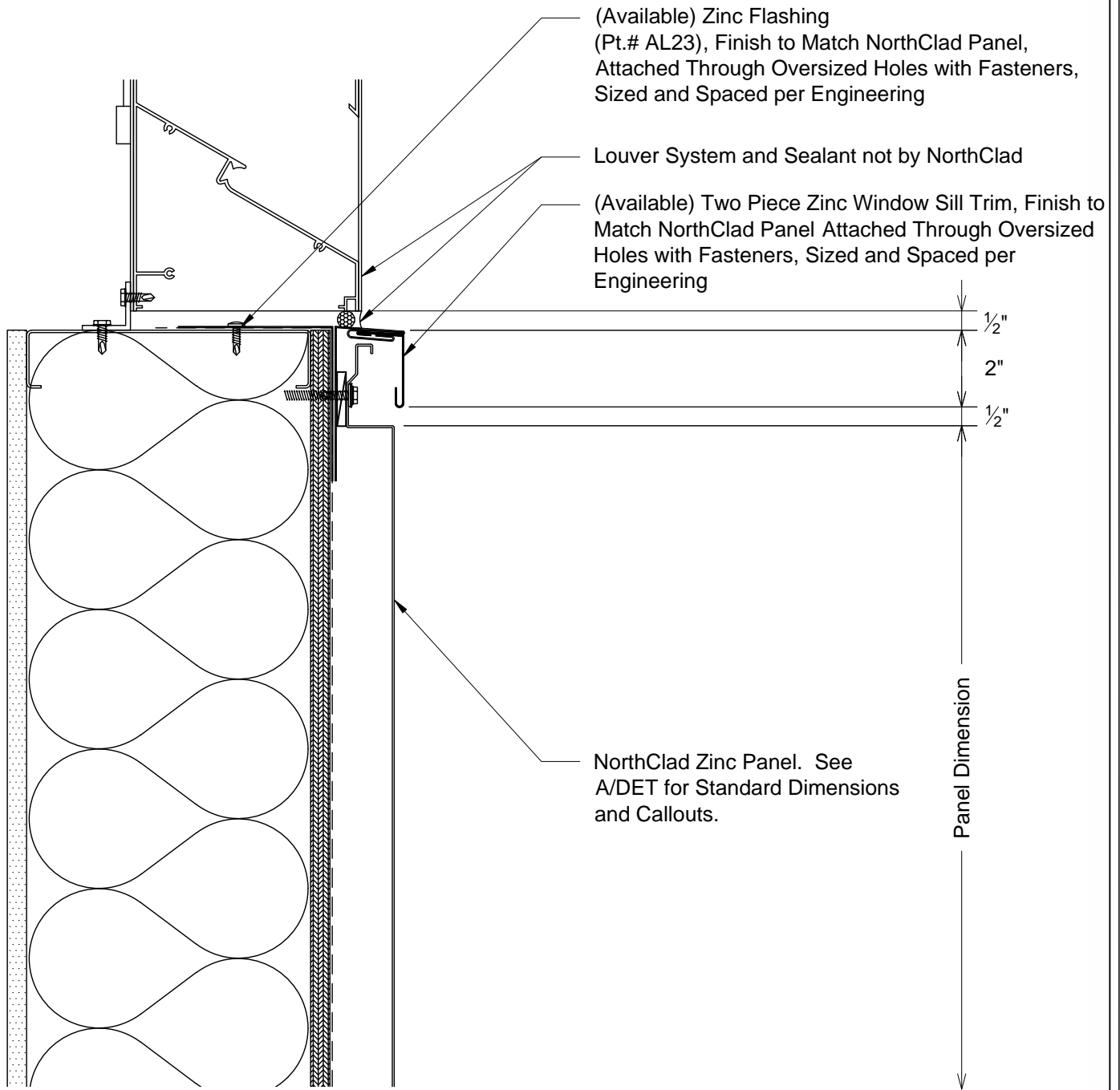
J2 Section - Louver Sill DET
