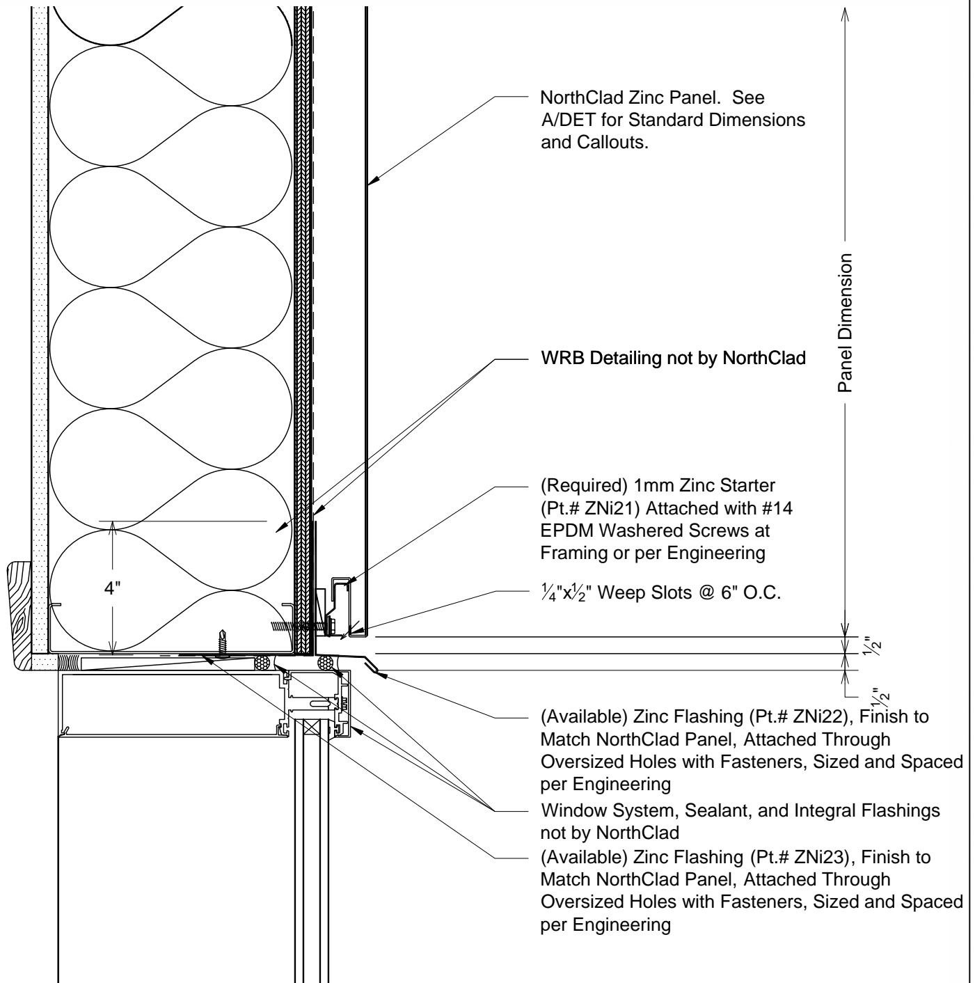
K1 Section - Window Head DET
