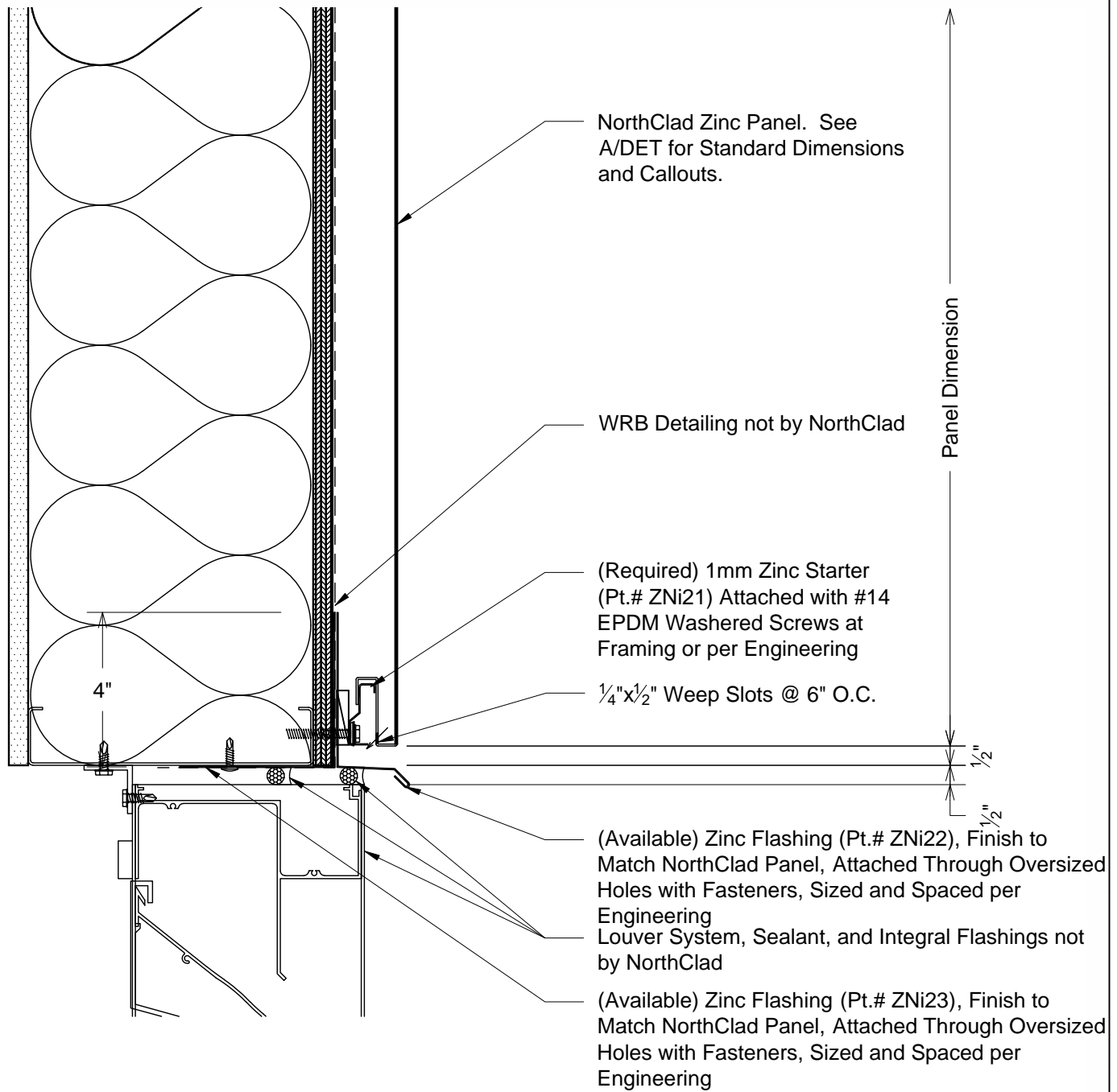
K2 Section - Louver Head DET
