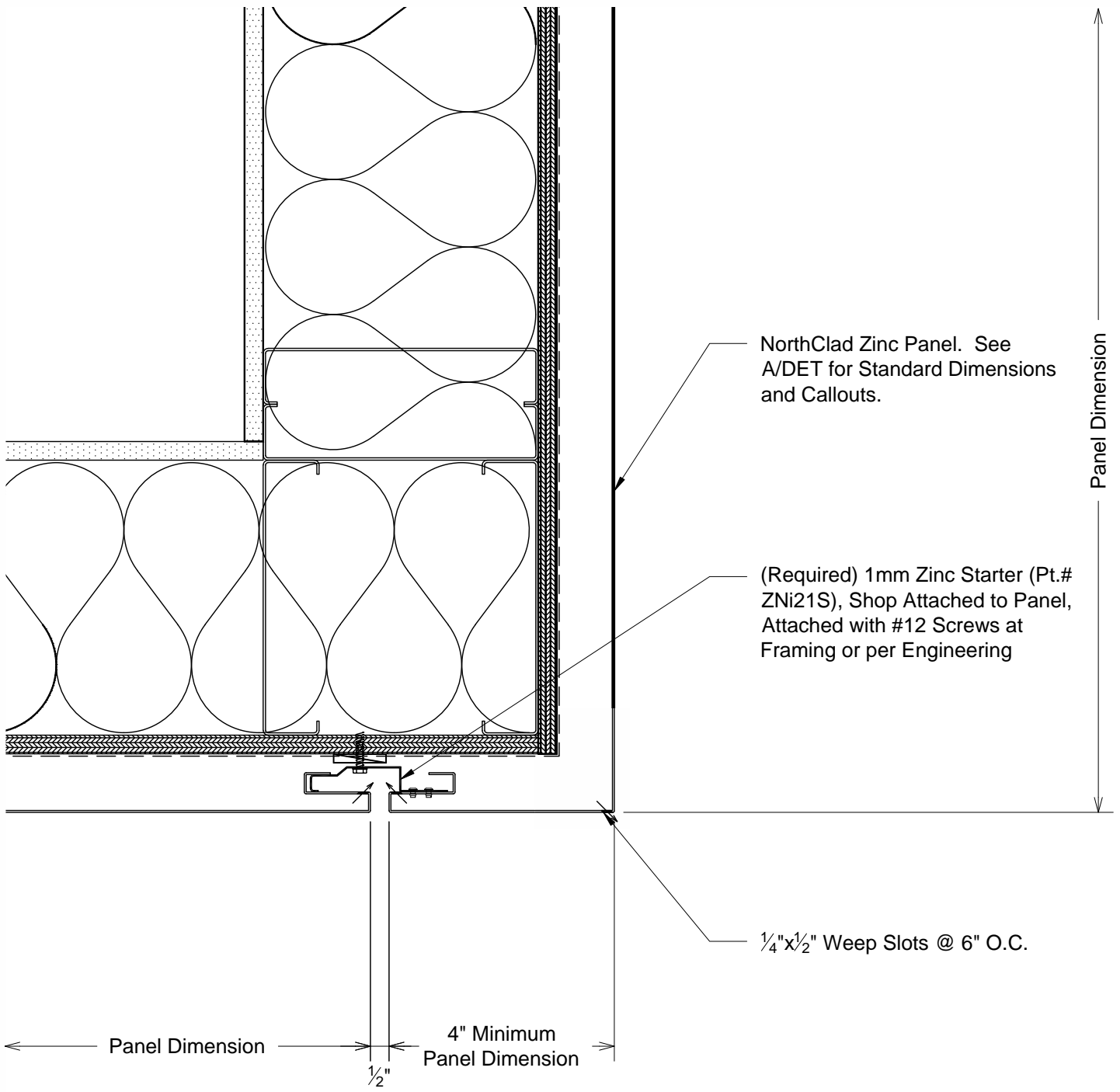
P1 Section - Fascia to Soffit DET
