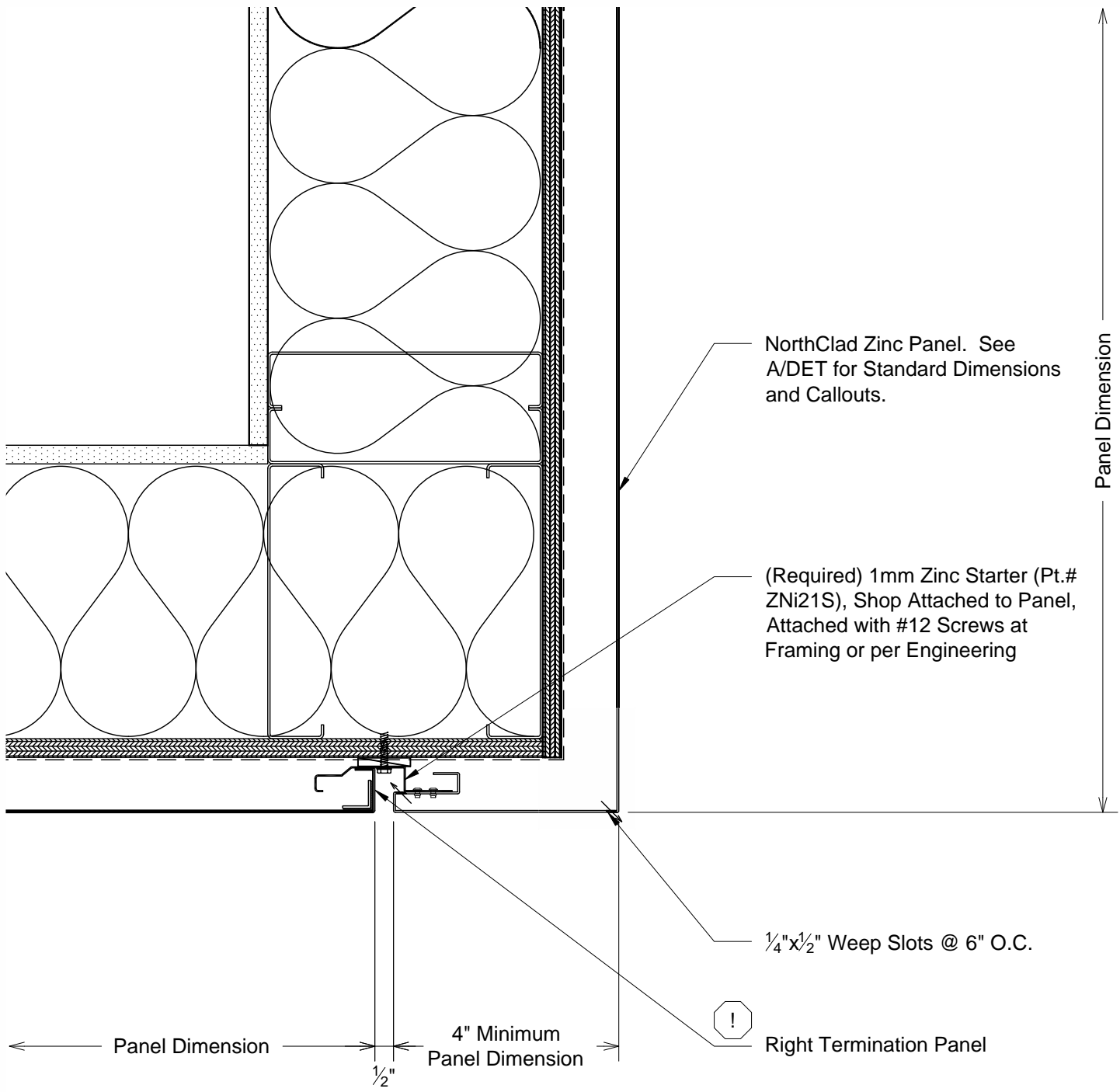
P2 Section - Fascia to Soffit DET
