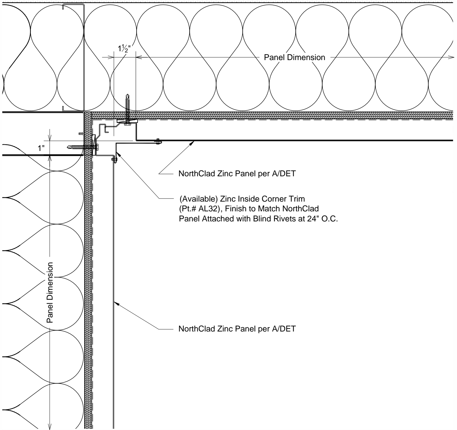
Q Section - Soffit at Top of Wall DET
