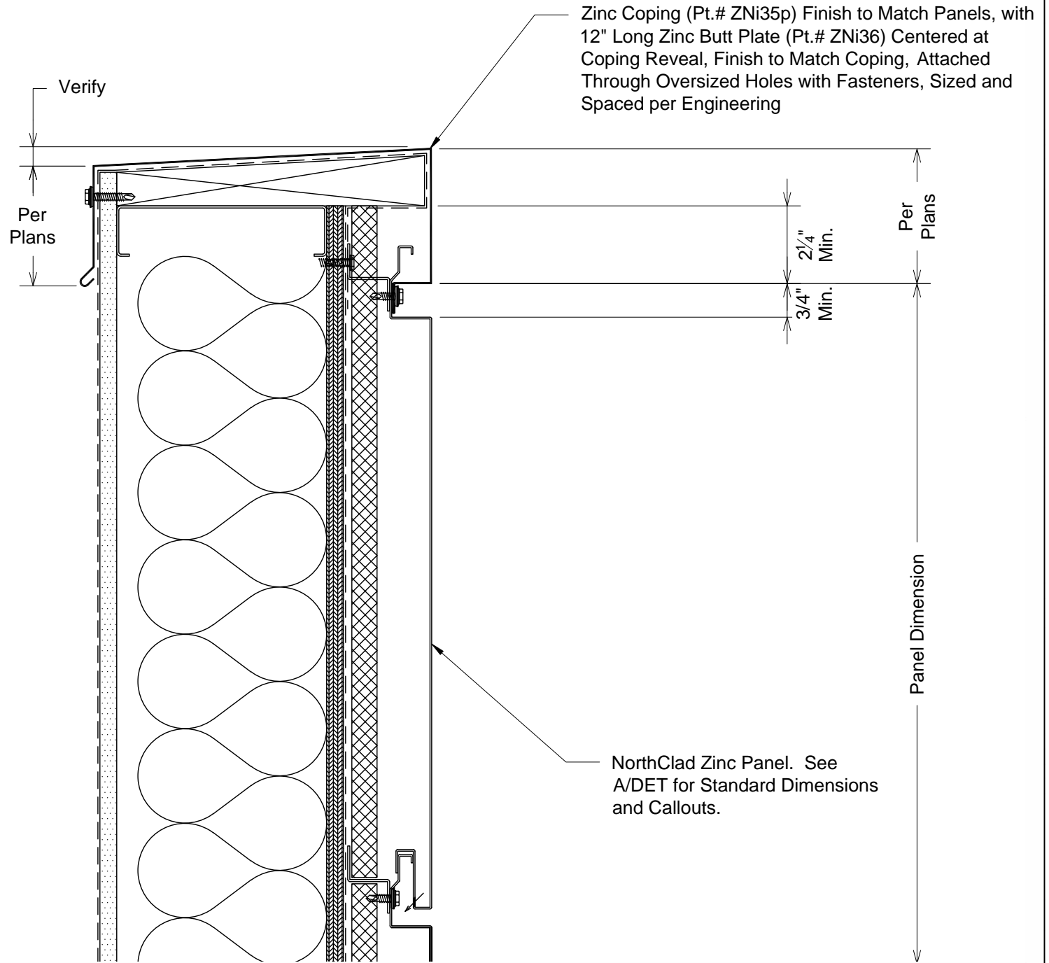
F Section - Formed Parapet Coping DET
