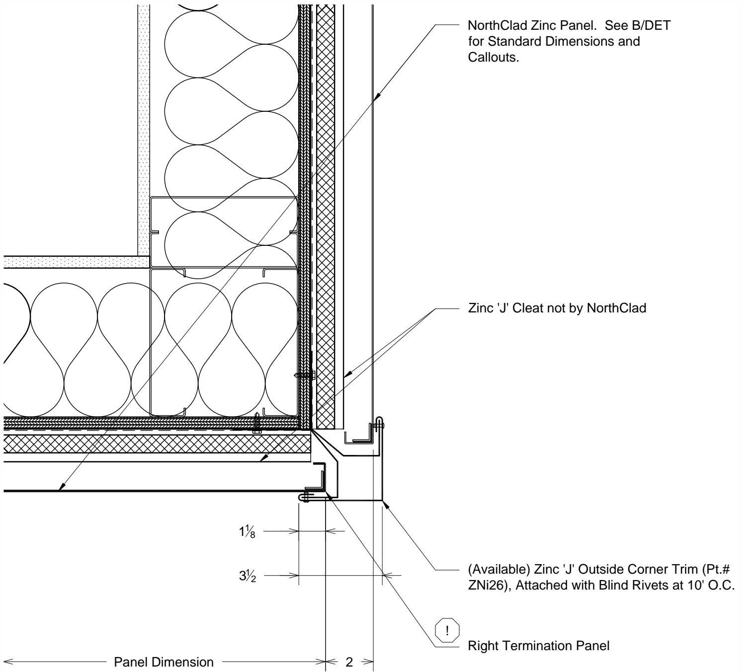
G2 Plan - Outside Corner with Trim DET
