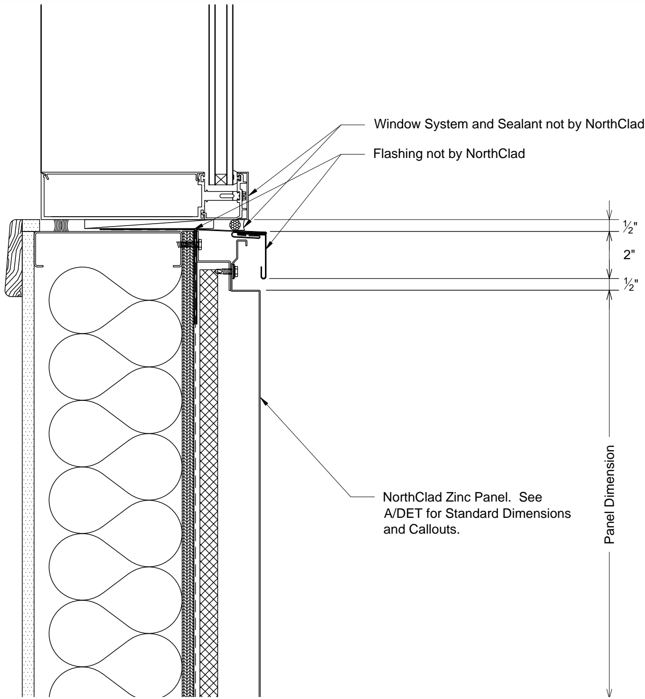
J1 Section - Window Sill DET
