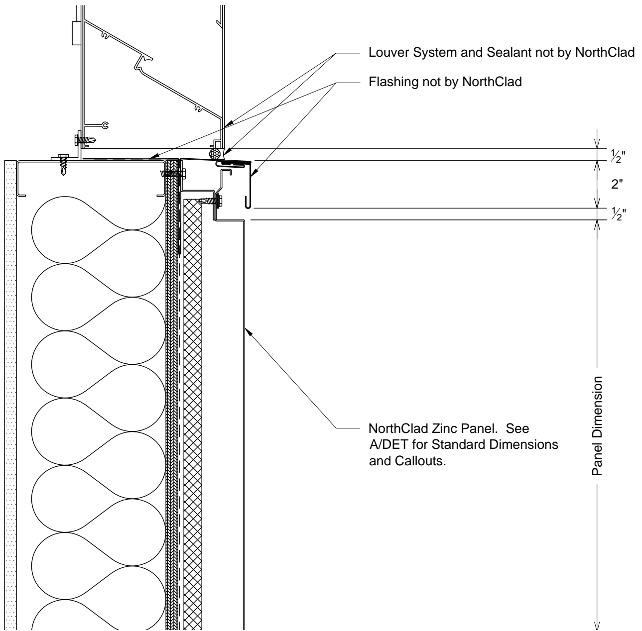
J2 Section - Louver Sill DET
