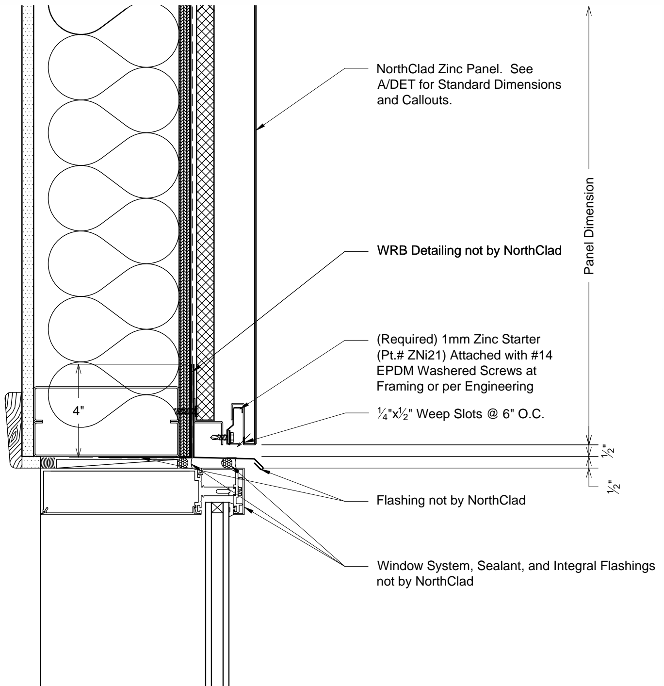
K1 Section - Window Head DET
