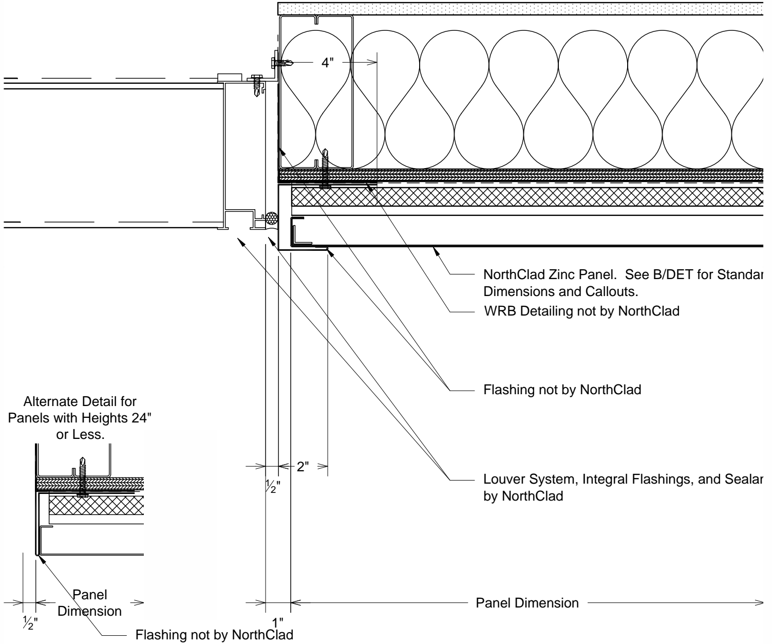
M2 Plan - Louver at Right Jamb DET
