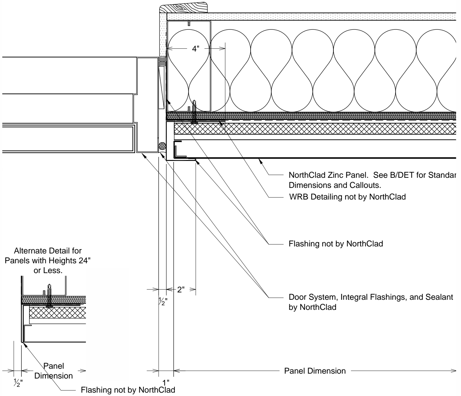
M3 Plan - Door at Right Jamb DET
