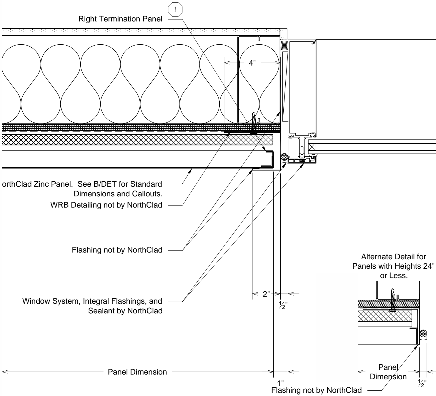
N1 Plan - Window at Left Jamb DET
