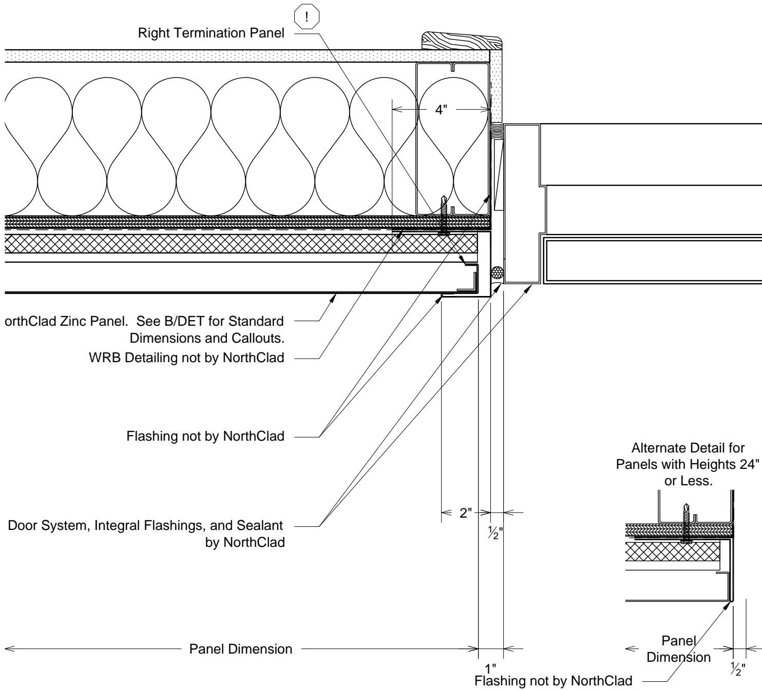
N3 Plan - Door at Left Jamb DET
