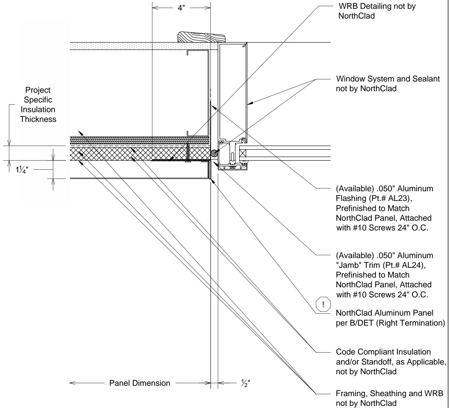
K1 DET Plan - Window at Left Jamb
