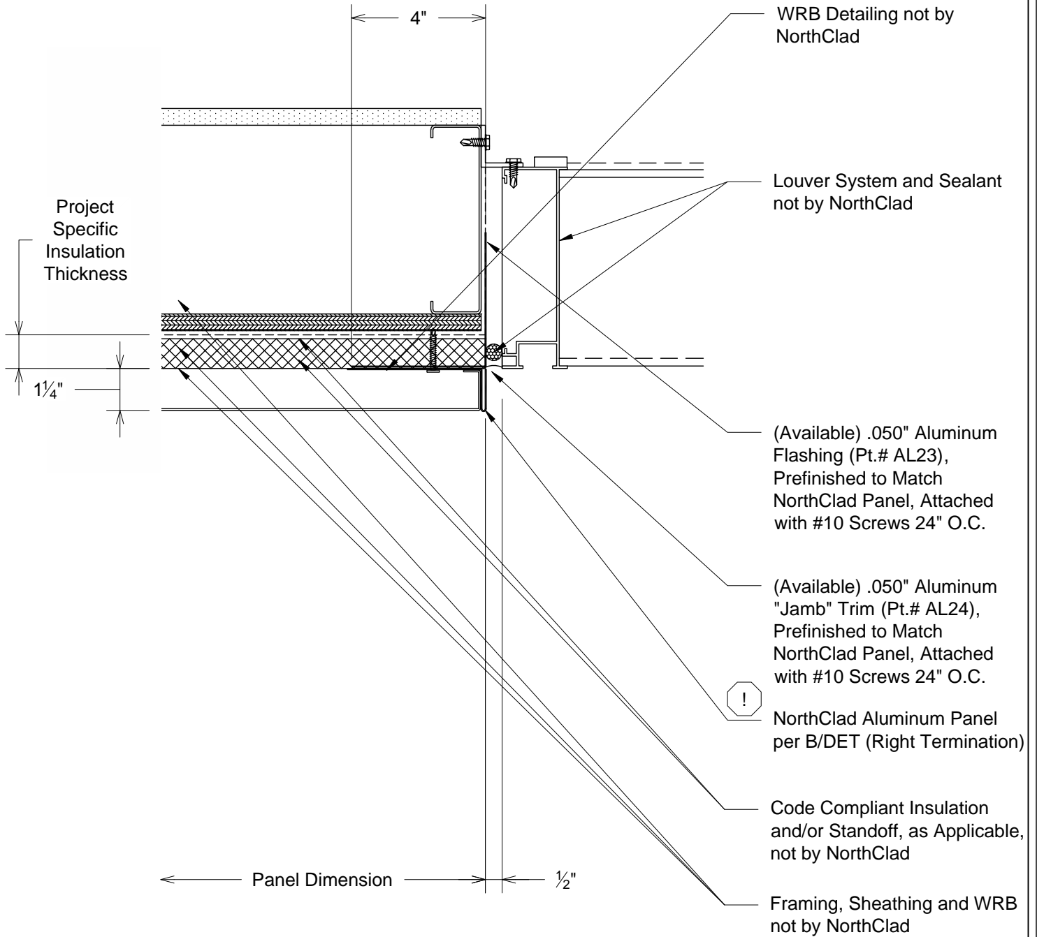
K2 DET Plan - Louver at Left Jamb
