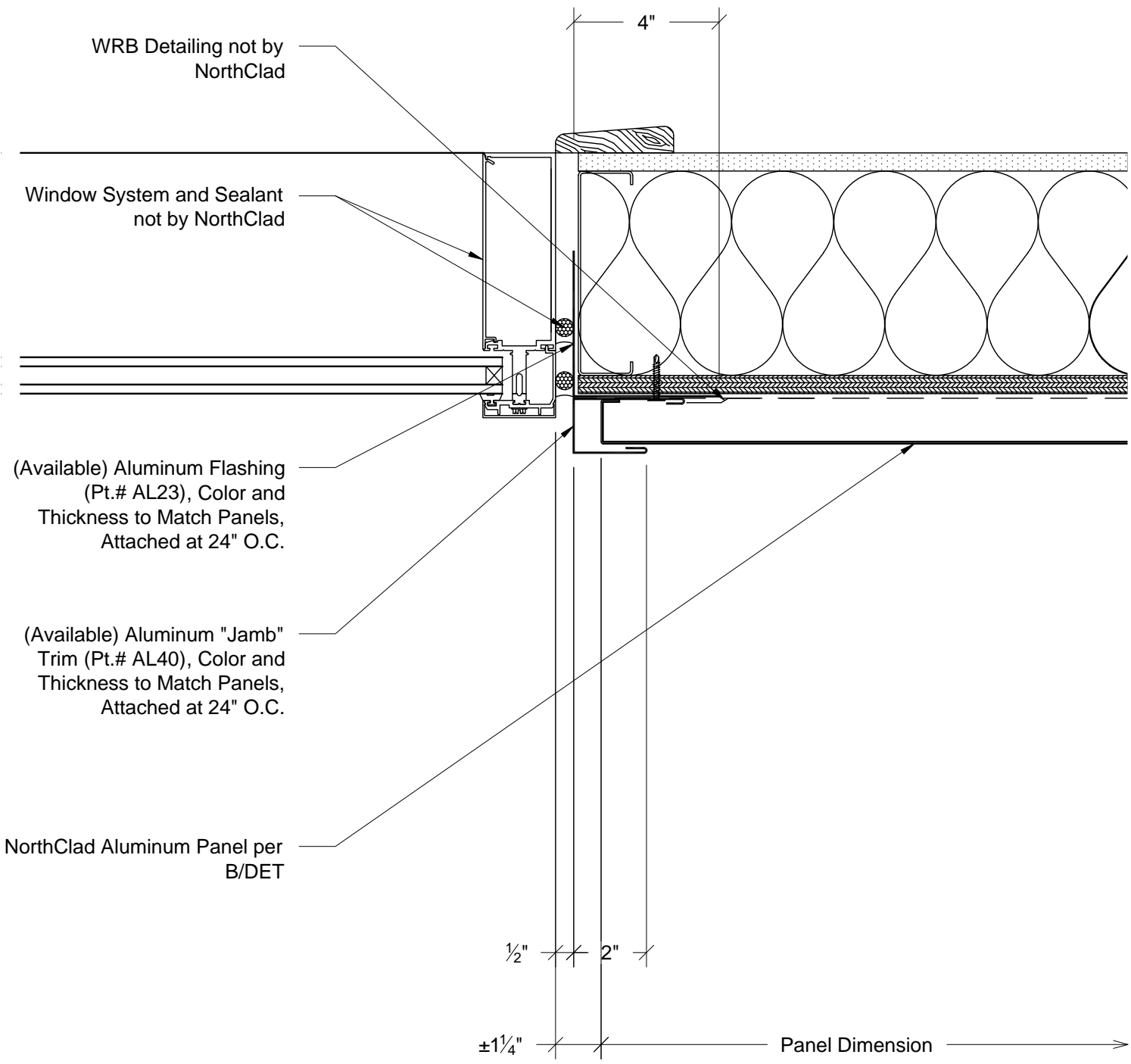
K1 Plan - Left Edge of Panel at Window Jamb System: AL Stacking with Inboard Insulation
