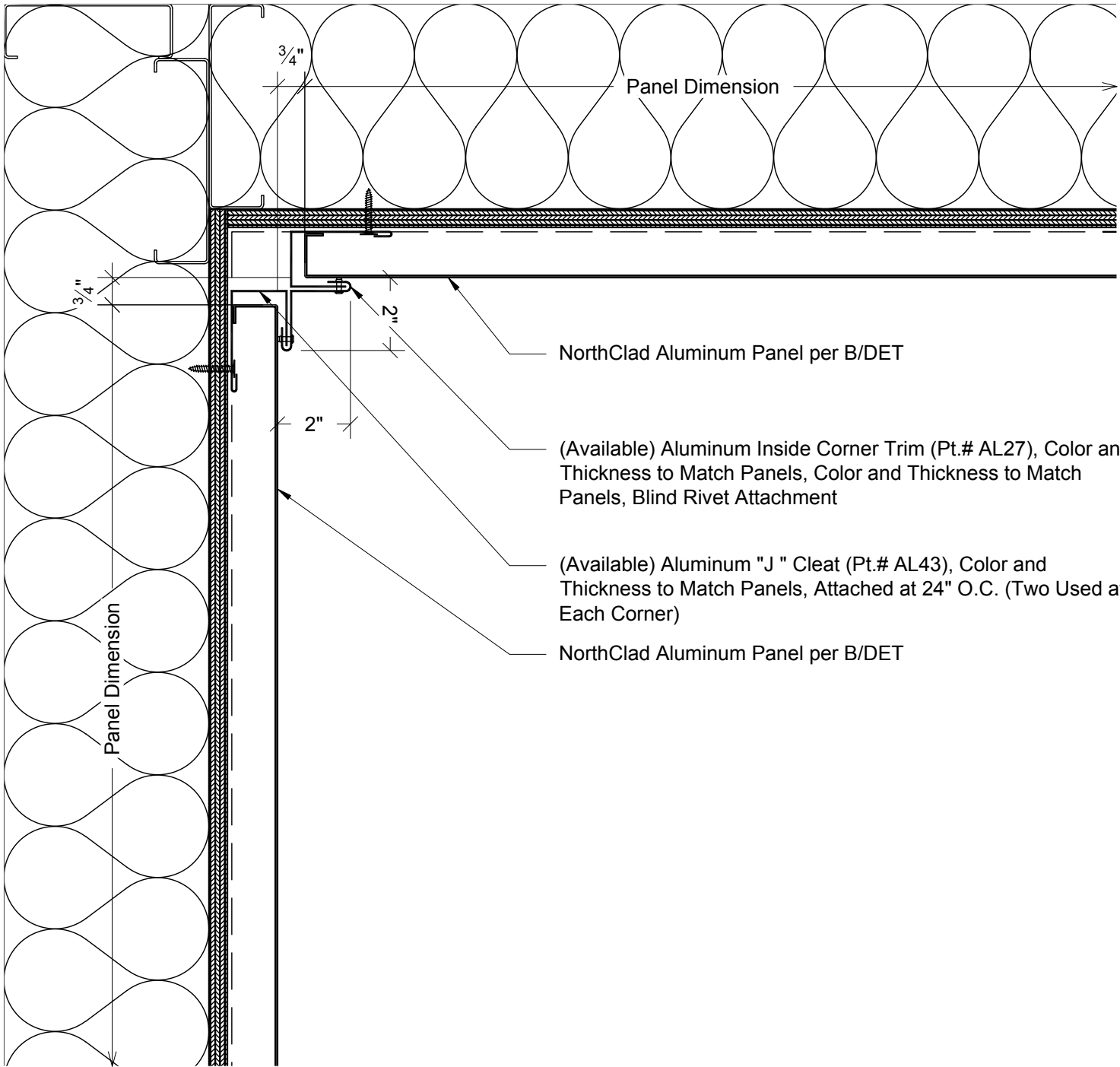
Plan - Edge of Panels at Inside Corner with Trim System: AL Stacking with Inboard Insulation
