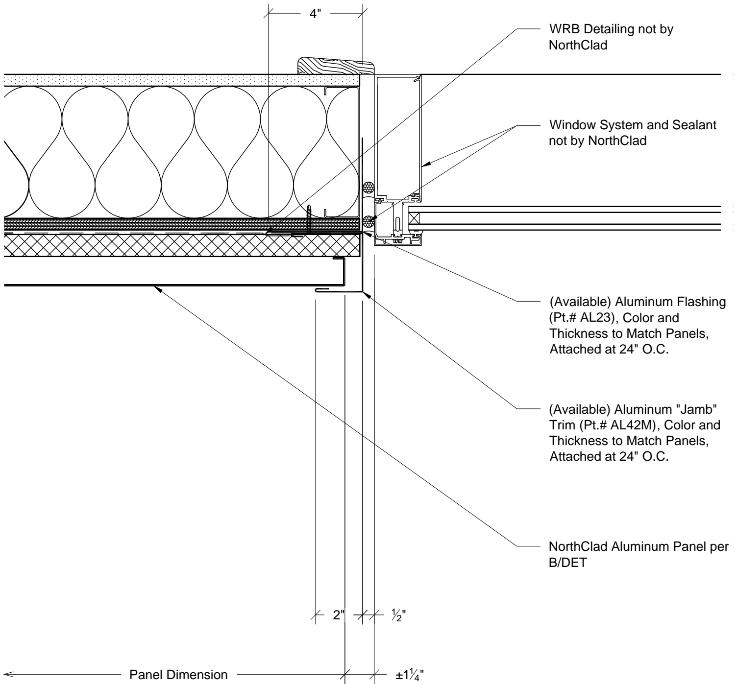
Plan - Right Edge of Panel at Window Jamb System: AL Stacking with Outboard Insulation
