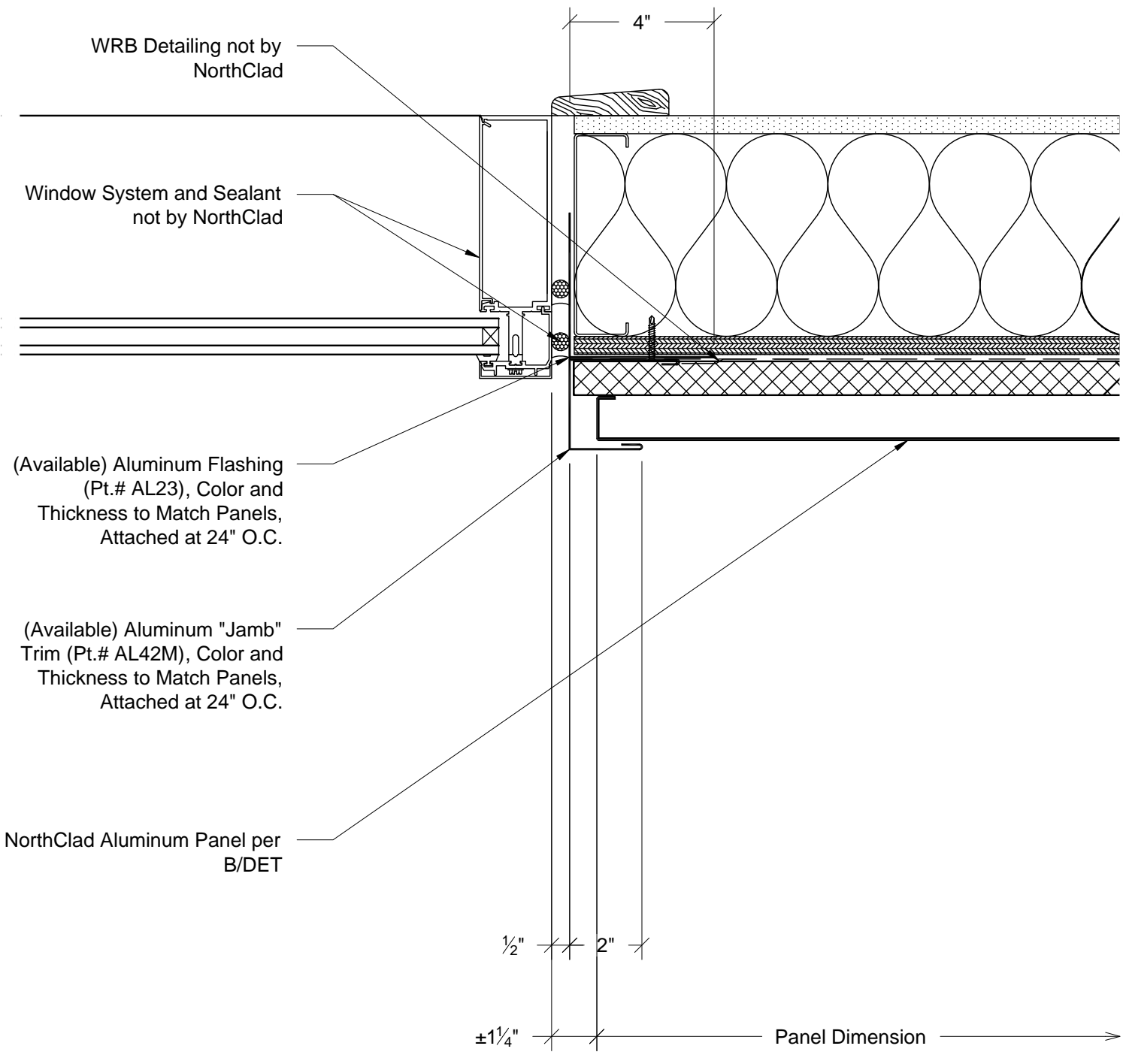
K1 Plan - Left Edge of Panel at Window Jamb System: AL Stacking with Outboard Insulation
