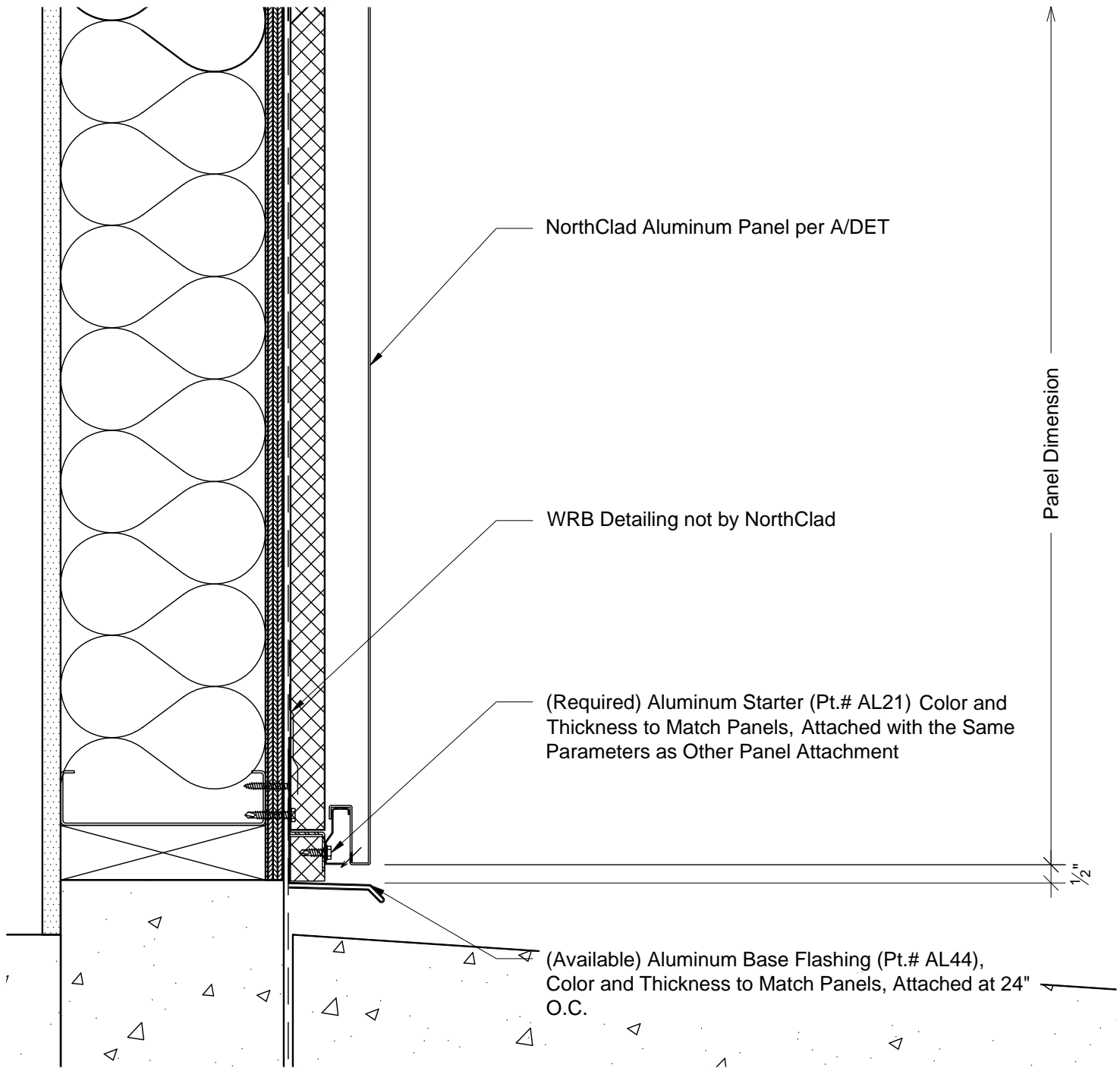
C Section - Bottom of Panel at Base of Wall System: AL Stacking with Outboard Insulation
