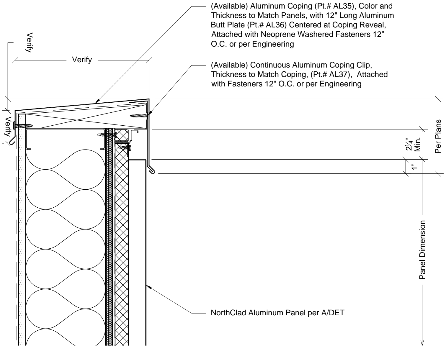
D Section - Top of Panel at Coping System: AL Stacking with Outboard Insulation
