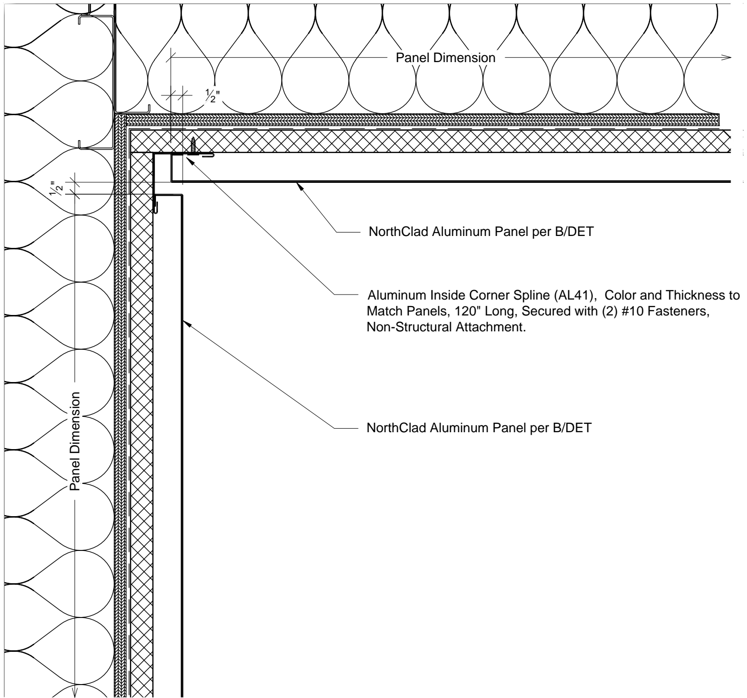
Plan - Edge of Panels at Inside Corner without Trim System: AL Stacking with Outboard Insulation
