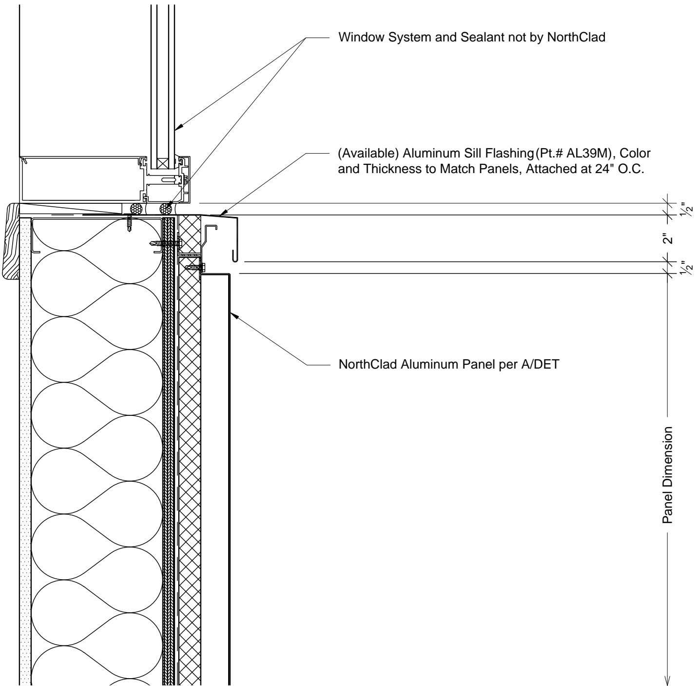
G1 Section - Top of Panel at Window Sill System: AL Stacking with Outboard Insulation
