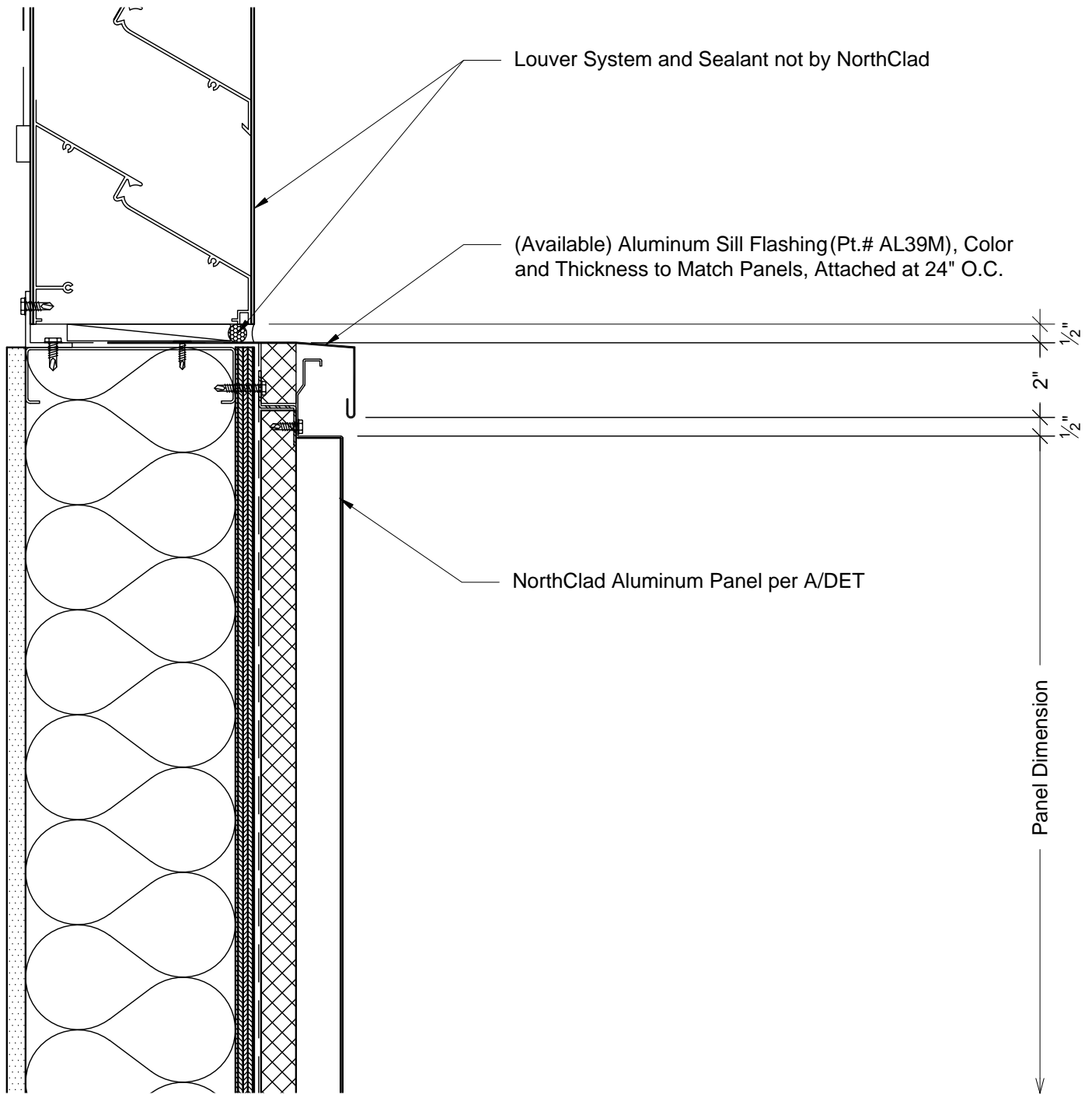
G2 Section - Top of Panel at Louver Sill System: AL Stacking with Outboard Insulation
