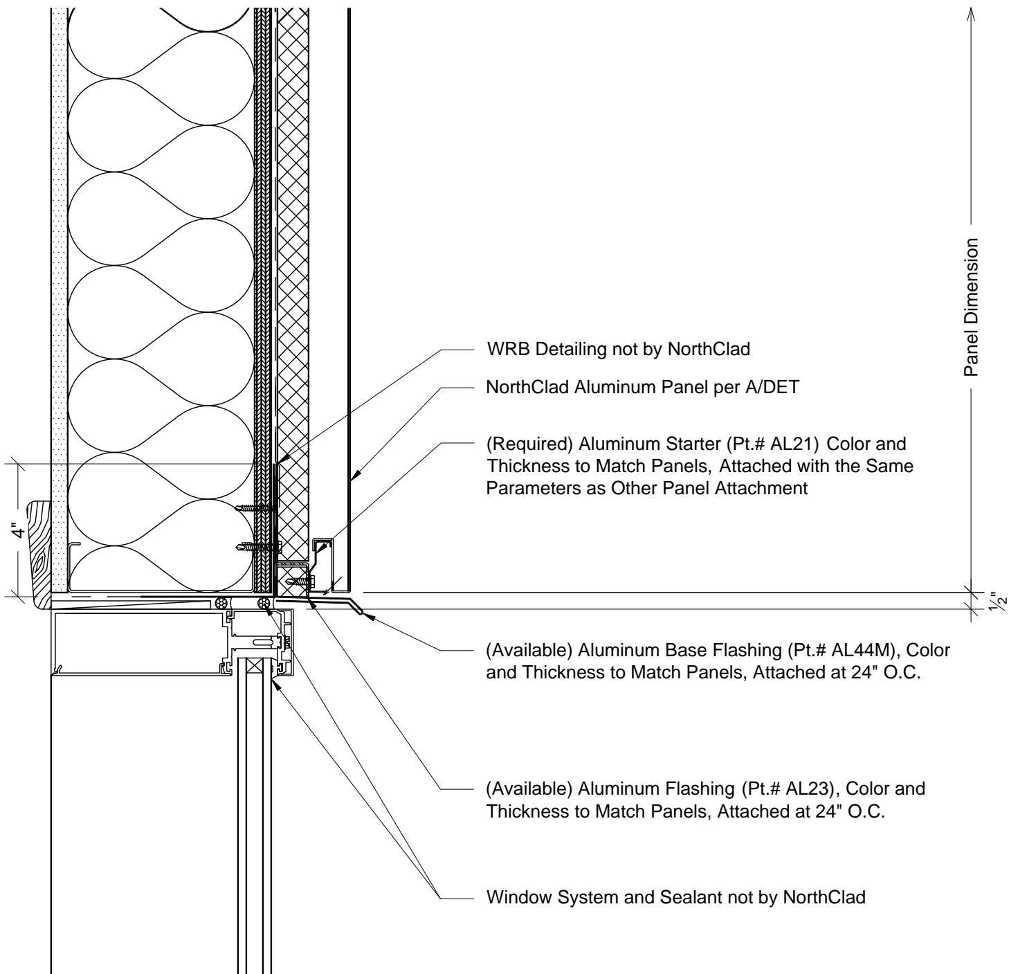
Section - Bottom of Panel at Window Head System: AL Stacking with Outboard Insulation
