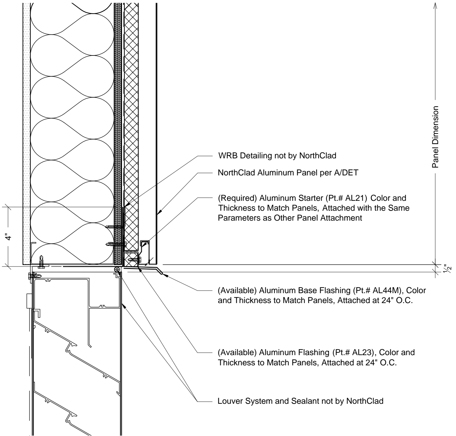
H2 Section - Bottom of Panel at Louver Head System: AL Stacking with Outboard Insulation
