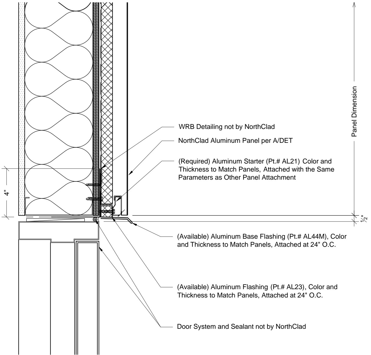
Section - Bottom of Panel at Door Head System: AL Stacking with Outboard Insulation
