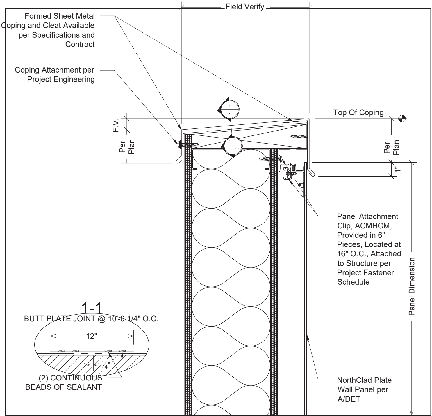
D2 Section - Top of Panel at Coping System: AL-PF with Inboard Insulation
