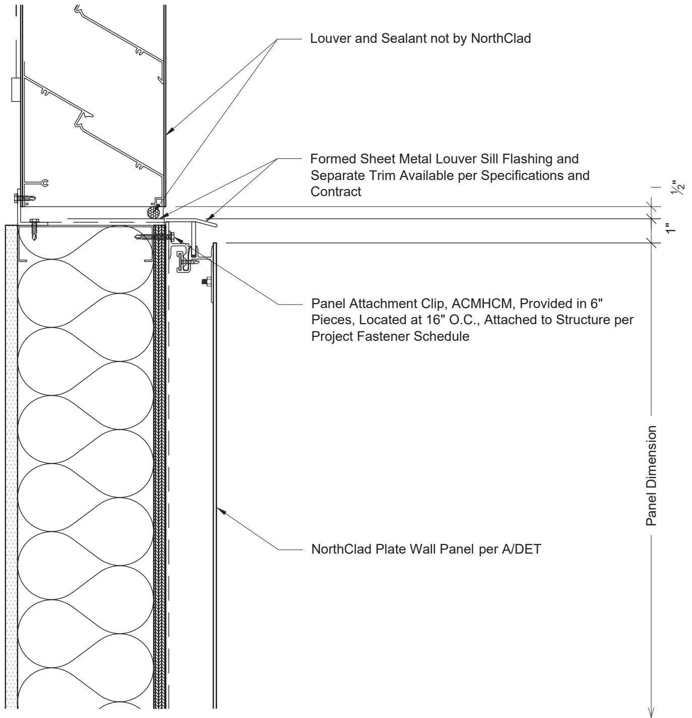
G2 Section - Top of Panel at Louver Sill System: AL-PF with Inboard Insulation
