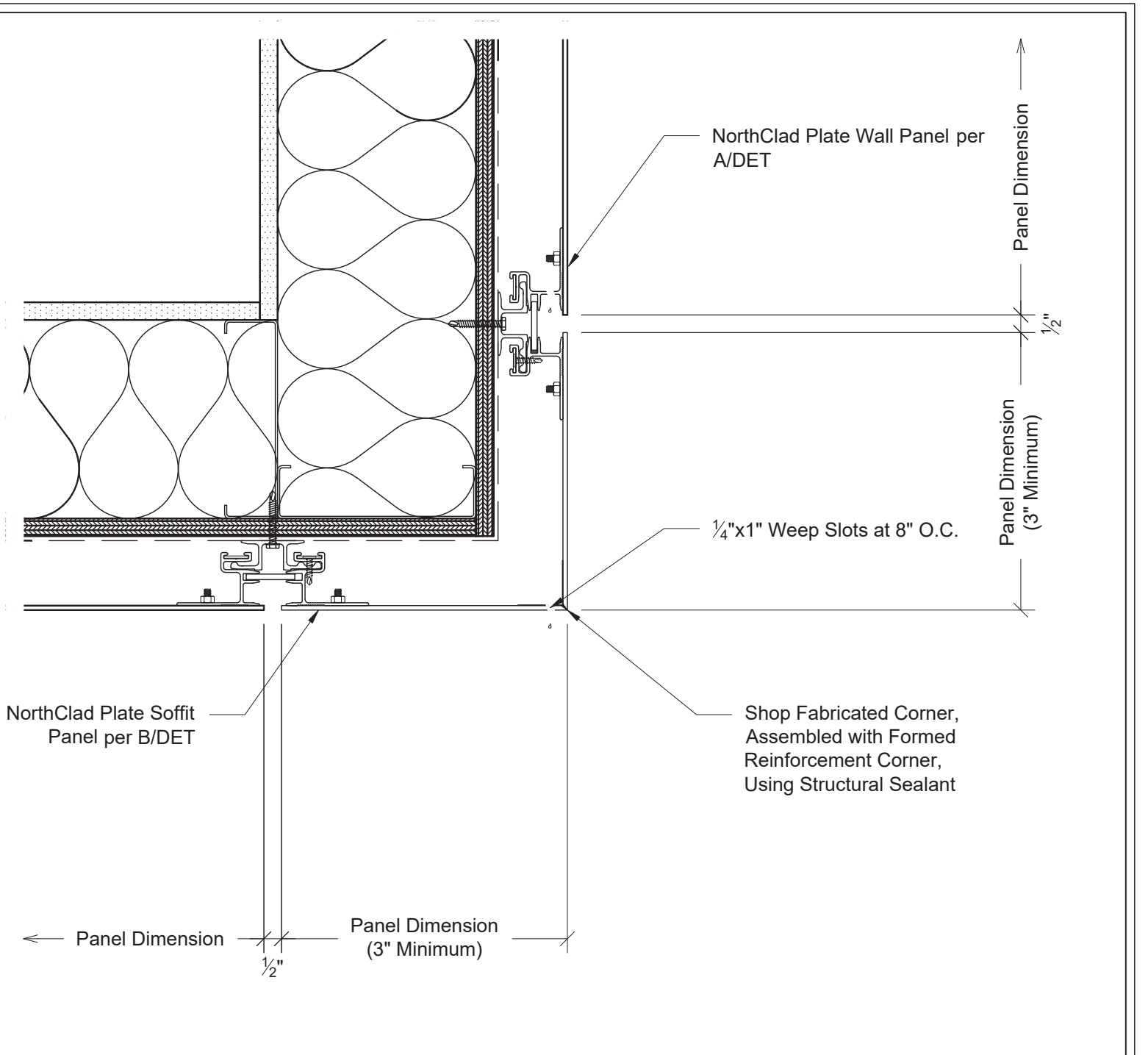
M1 Section - Panels at Fascia to Soffit Transition System: AL-PF with Inboard Insulation
