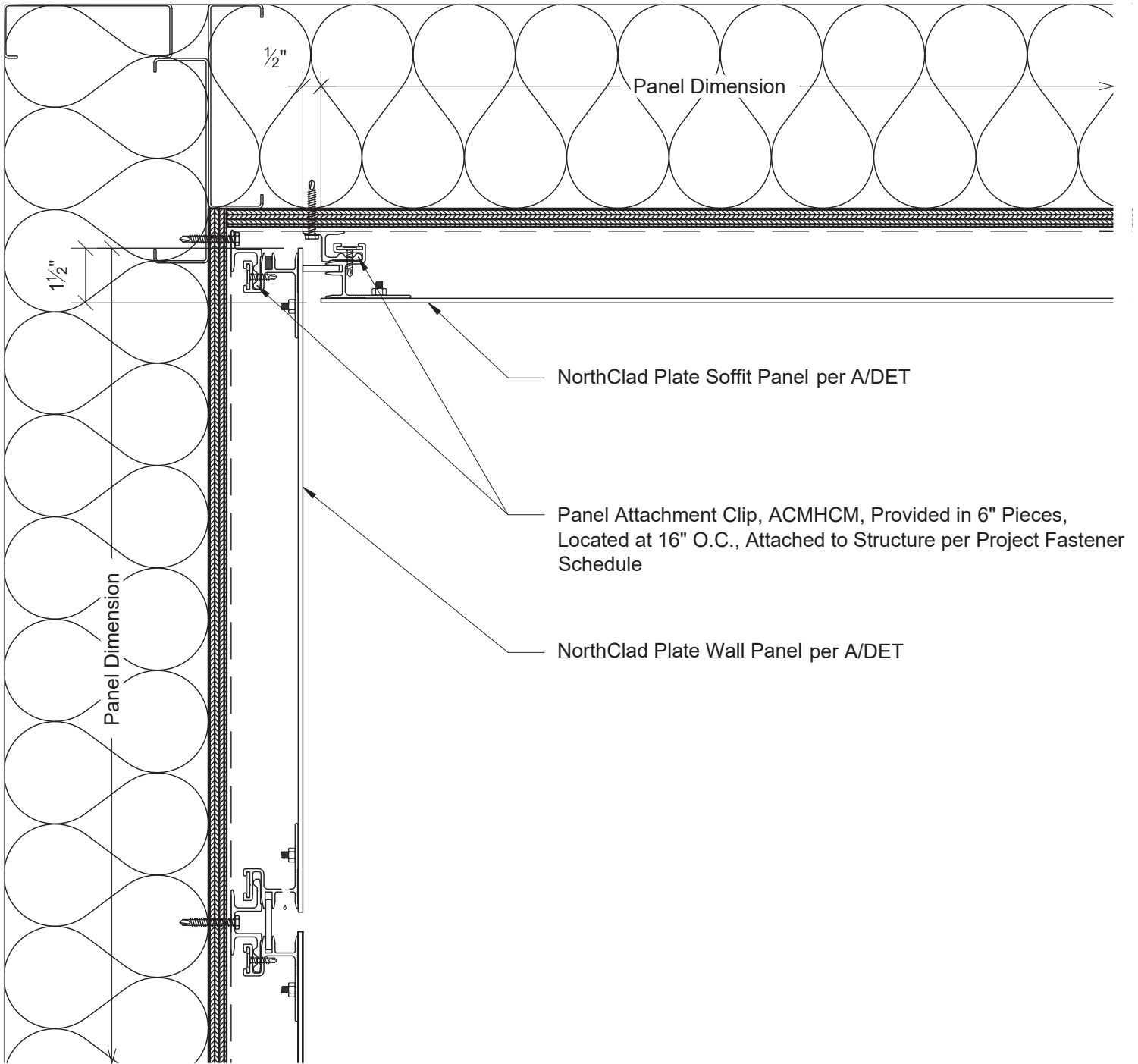
N1 Section - Panels at Wall to Soffit Transition System: AL-PF with Inboard Insulation
