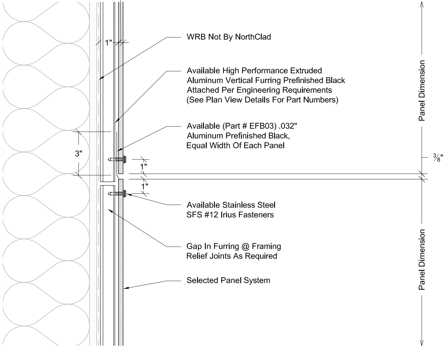
A Section - NorthClad EF - Horizontal Joint DET REFERENCE: NorthClad EF System
