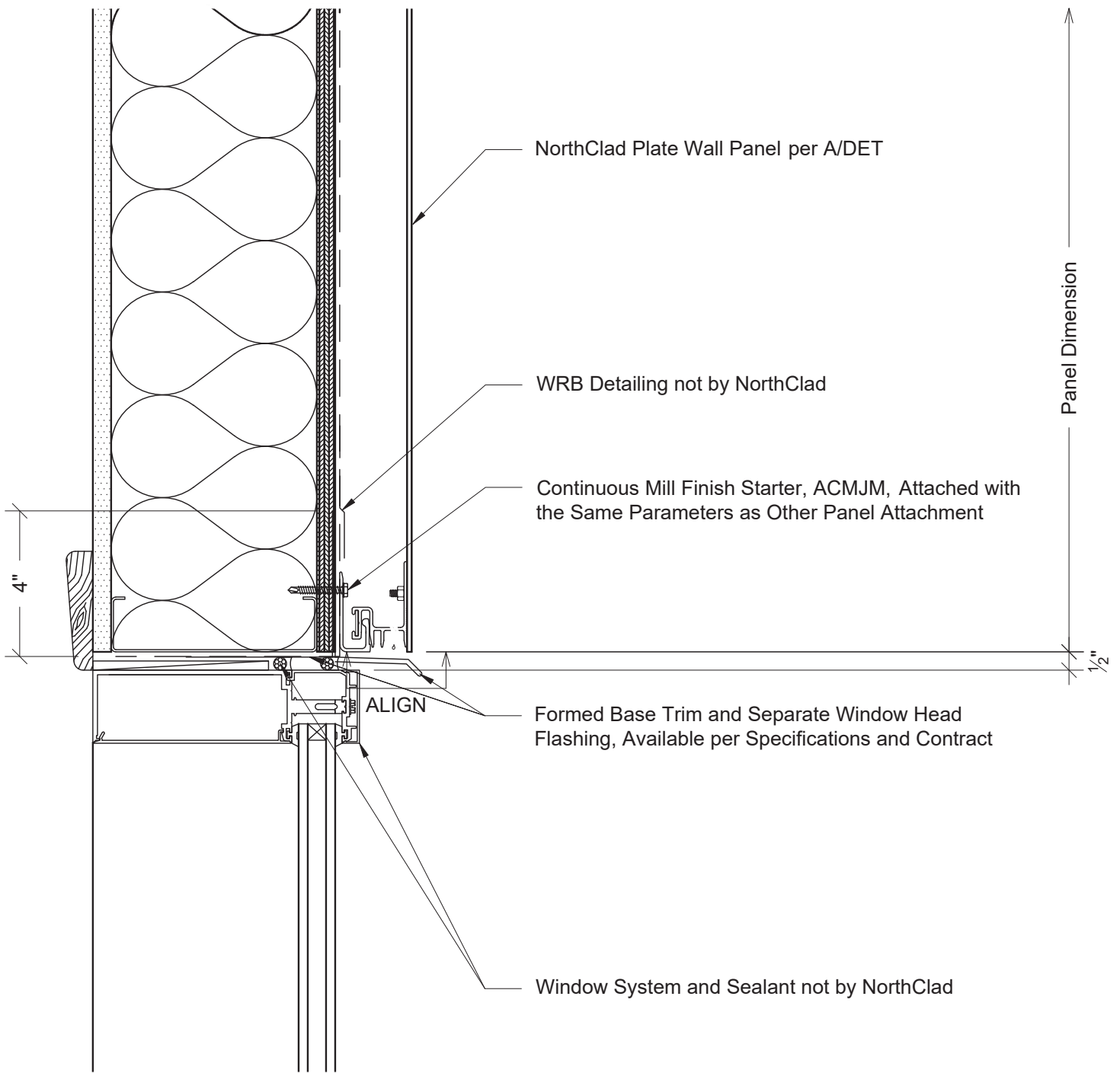
Section - Bottom of Panel at Window Head System: AL-PF with Inboard Insulation
