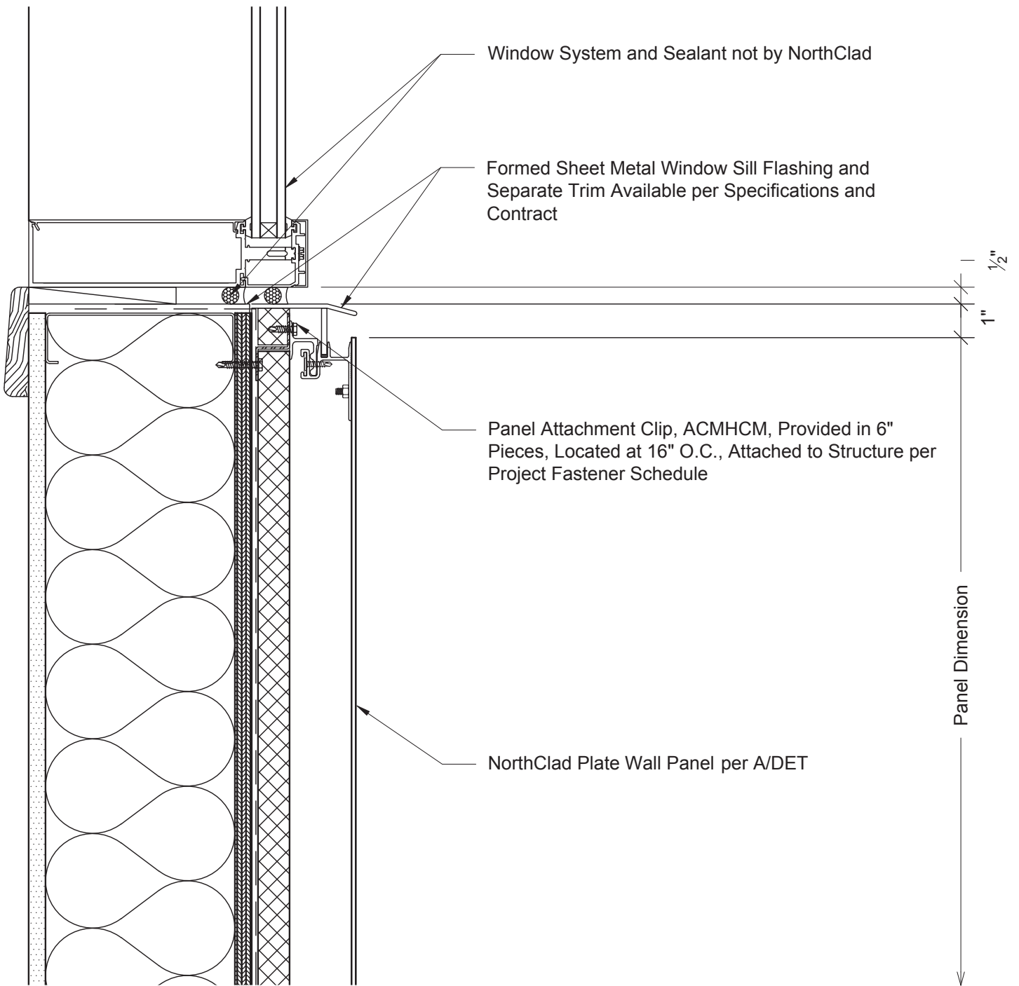
G1 Section - Top of Panel at Window Sill System: AL-PF with Outboard Insulation
